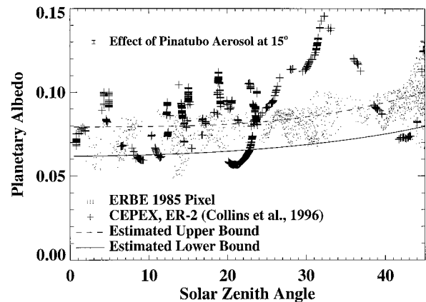
FIG. 6. Clear-sky TOA albedo: The + marks indicate ER-2 broadband albedo measurements from the tropopause, corrected to reflect TOA albedos. They have been screened for clear sky by separate, nadir viewing instruments. The points are ERBE pixel data for the central Pacific ( 0^\circ\text{--}5^\circ\text{S} ; 165^\circ\text{E}\text{--}165^\circ\text{W} ) from March 1985, corrected to simulate the presence of the stratospheric aerosol observed during 1993. The magnitude of the corrections is shown as a range bar. Two lines are shown that represent our upper and lower estimates of clear-sky albedo. The upper estimate is taken from the ERBE March 1986 gridded mean albedo (the highest of the five ERBE years), and the lower estimate is taken from Collins et al. (1996). (There are still data below the lower estimate to allow for natural variability.)
