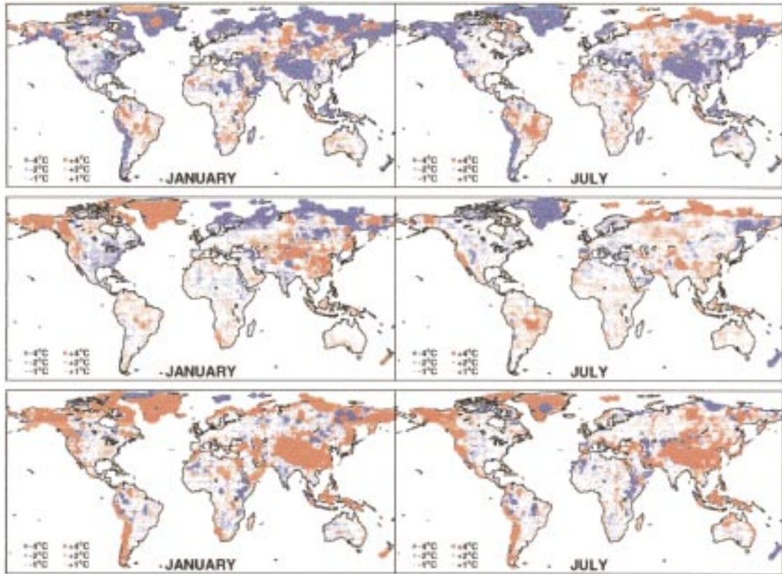
FIG. 22. Differences between CRU, LEG, and CRA (degraded to 2^{\circ} lat \times 2^{\circ} long) mean temperature grids for January and July. The size of the dots (continuous scale) indicates the magnitude of the differences as shown in the legend. Top CRU minus LEG, middle CRU minus CRA, and bottom LEG minus CRA.
