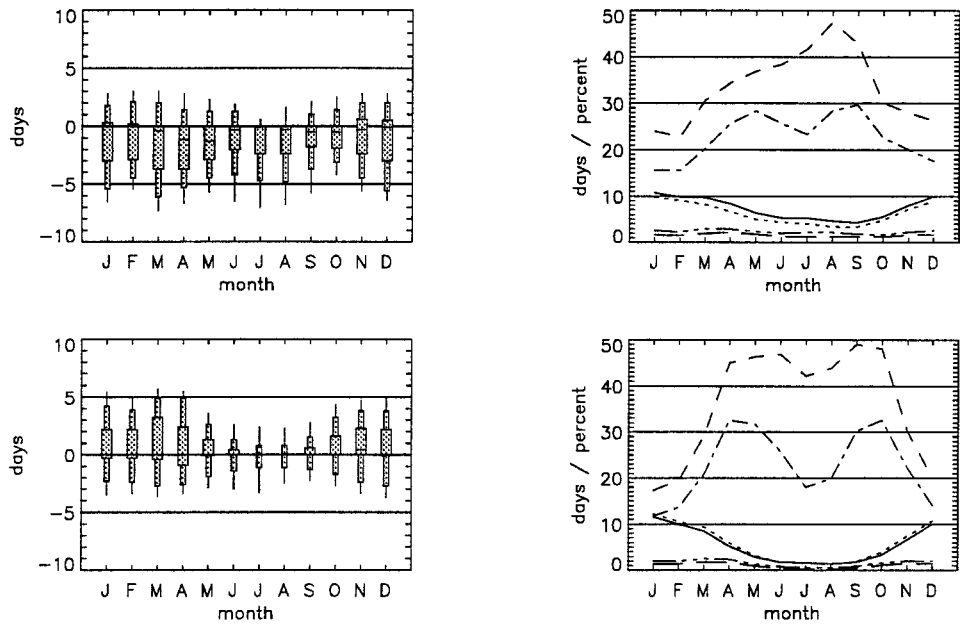
FIG. 13. (top) Validation statistics for the air frost and minimum temperature to ground frost and (bottom) the minimum temperature only to ground frost conversions. See Fig. 5 for explanation.
