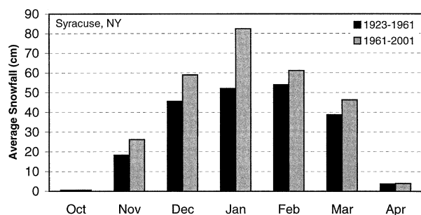
FIG. 8. Oct–Apr average monthly snowfall for Syracuse, NY, for the periods 1923–61 and 1962–2001.
