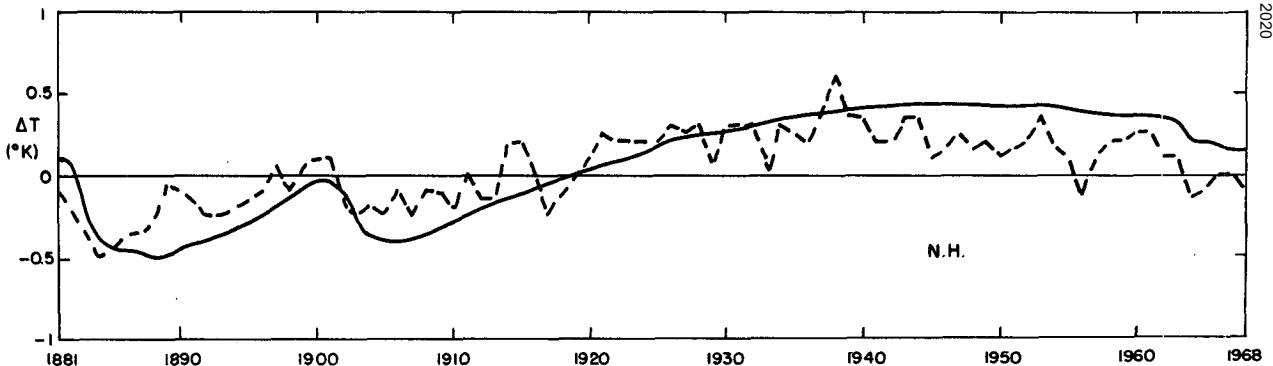
FIG. 13. Results of Mitchell volcanic dust simulation run (9) (solid curve) compared with observations of Budyko-Asakura (dashed curve).
