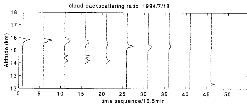
FIG. 3. Cloud observation in the evening of 18 July 1994. A cloud in the tropopause and a cloud in the upper troposphere were simultaneously observed.
