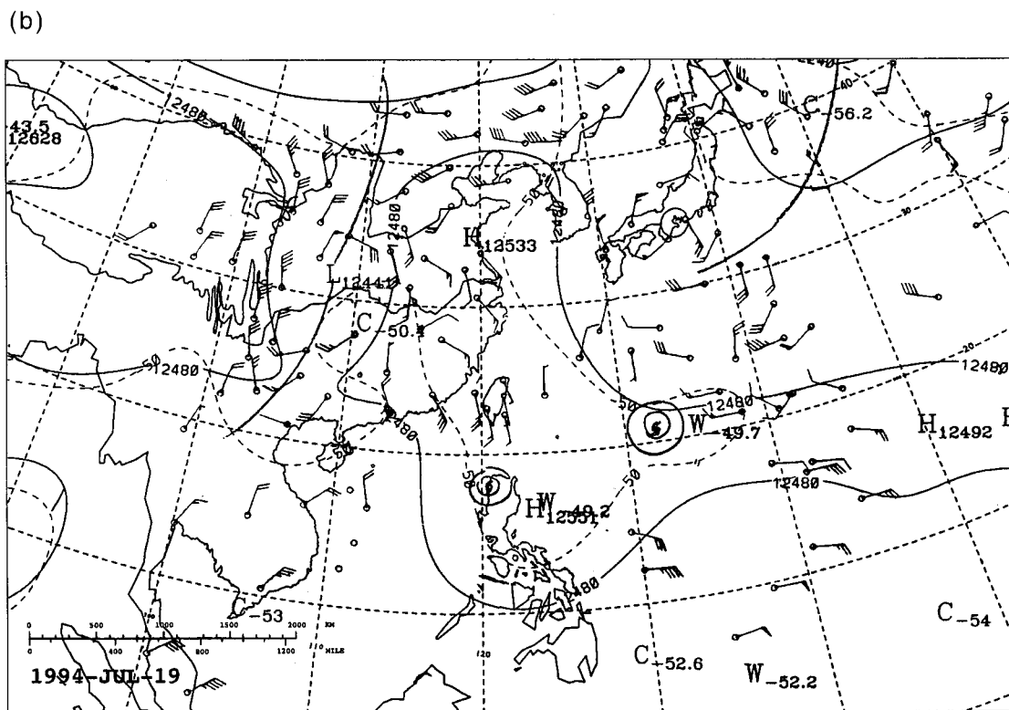
FIG. 7. (a) Upper-air map at 200 hPa, 0800 LST 14 May (0000 UTC) 1994. (b) Upper-air map at 200 hPa, 0800 LST 19 July (0000 UTC) 1994.
