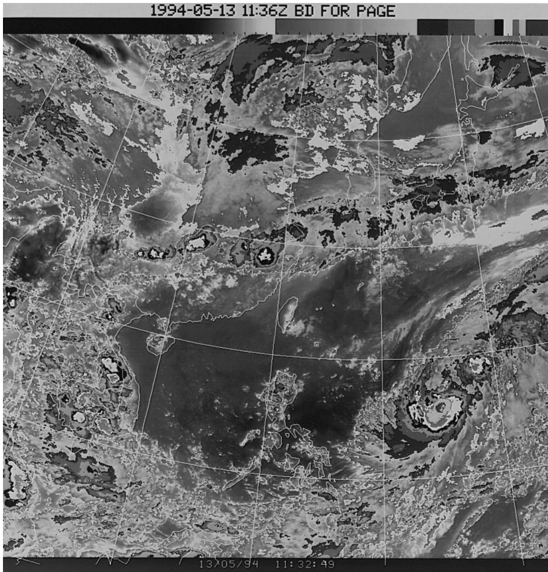
FIG. 8. GMS infrared satellite picture on 13 May 1994.
