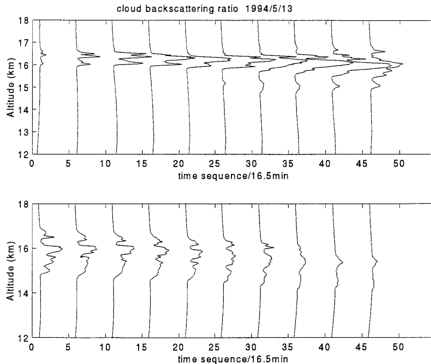
FIG. 1. Time sequence for cirrus cloud detected on 13 May 1994. The cloud profiles are expressed in two columns where the lower column is continued from the upper column. The cloud started at 2320 LST and disappeared toward daybreak. Each profile resulted from integration of data for 16.5 min and was plotted with the backscattering ratio progressively offset by 5.
