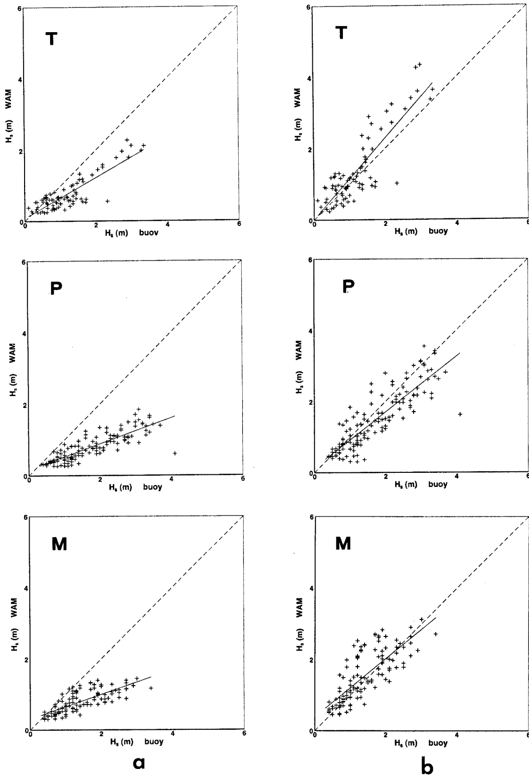
FIG. 7. (a) Scatterplots of the results obtained using the model wind (see Fig. 6) and (b) the same after the wind enhancement.
