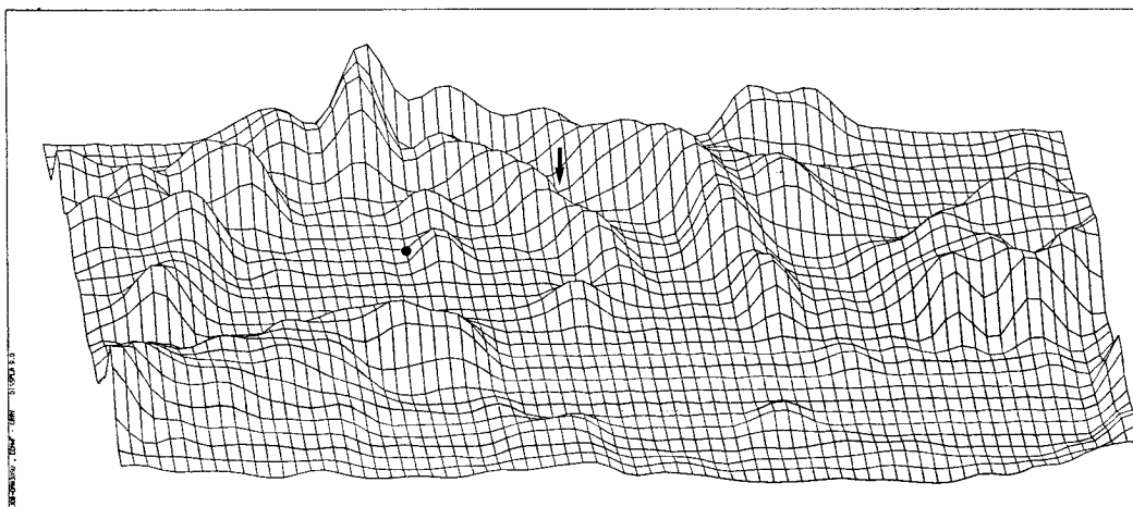
FIG. 2. The orography of the Mediterranean Sea as represented in the T213 spectral model. The dot shows the position of Alghero (see Fig. 1). The arrow indicates the Adriatic Sea.
