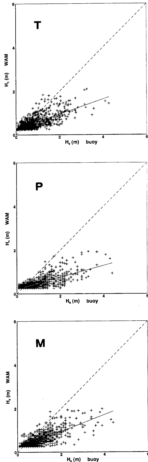
FIG. 4. Scatterplot of the model vs measured wave height for 1992 at the three positions shown in Fig. 3.
