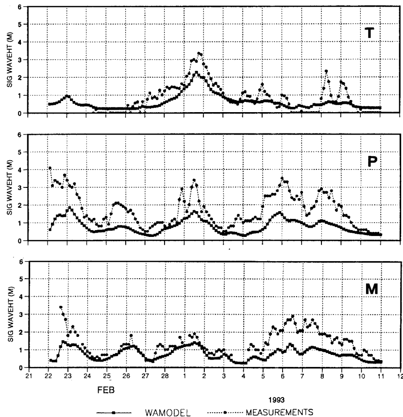
FIG. 6. Time series of the modeled and measured wave height at the three positions shown in Fig. 5 during the storm of February–March 1993.
