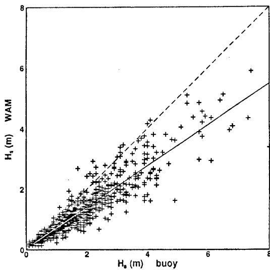
FIG. 1. Scatterplot of the model vs measured wave height at Alghero, on the west coast of Sardinia. The position is shown in Fig. 2.
