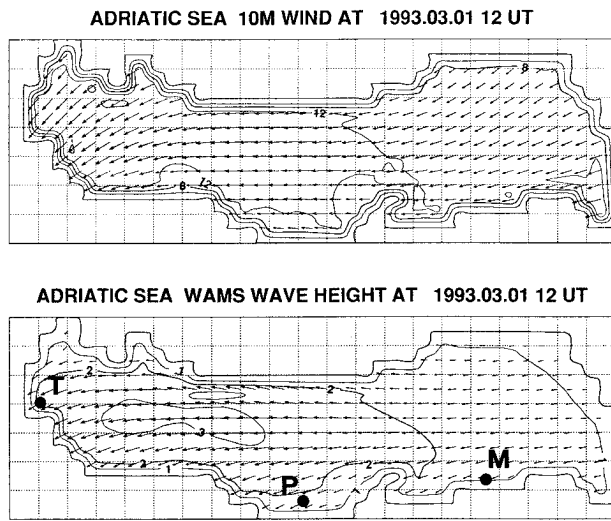
FIG. 5. Wind and wave situations on the Adriatic Sea (as seen by the model) at 1200 UTC 1 March 1993. The dots show the positions where wave-measured data are available (T—tower, P—Pescara, M—Monopoli).
