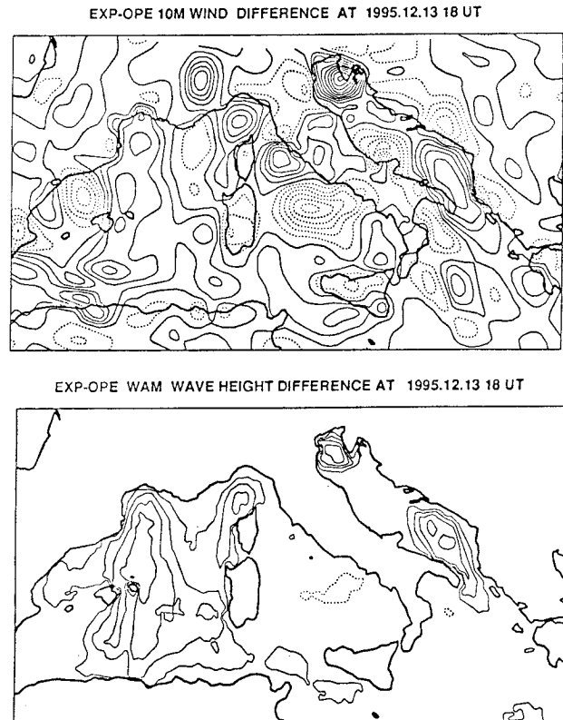
FIG. 14. With reference to Fig. 13a wind speed differences obtained with reduced and normal horizontal diffusion. Isolines at 20 \text{ cm s}^{-1} interval. Continuous lines represent positive values; dotted lines are for negative ones. (b) As in (a) but for wave height. Isolines at 5\text{-cm} interval. (After Cavaleri et al. 1997.)
