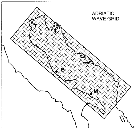
FIG. 3. The grid fitted to the Adriatic Sea. The dots show the positions where wave-measured data are available (T—tower, P—Pescara, M—Monopoli).
