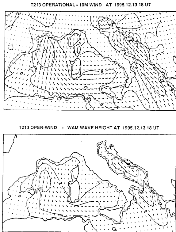
FIG. 13. Wind and wave fields in the western Mediterranean Sea at 1800 UTC 13 December 1995.
