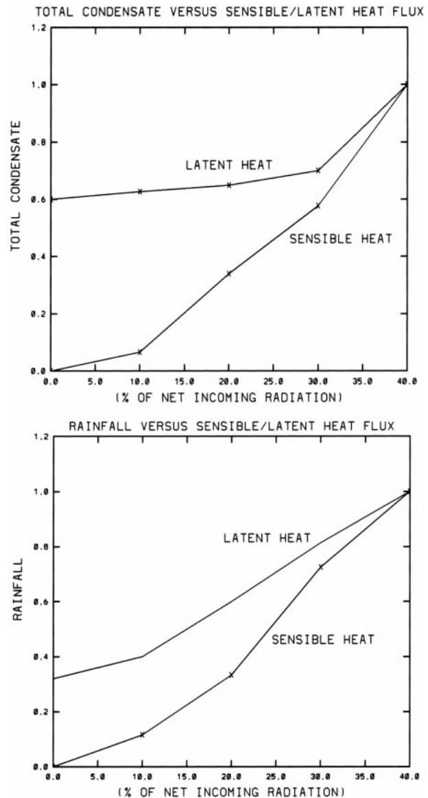
FIG. 12. (a) Total condensate vs sensible and latent heat flux. (b) Accumulated rainfall vs sensible and latent heat flux.
