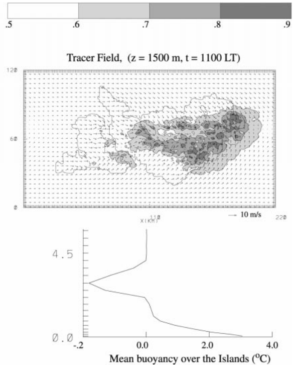
FIG. 5. (a) Concentration of tracer field at z = 1500 m overlaid on surface vector field ( t = 1100 LT). Initially, the tracer field is horizontally homogenous with a value of one at the surface, linearly decreasing to zero at 3 km. (b) Vertical profile of mean buoyancy field above the Tiwi Islands. Note that the scale on the negative side has been expanded by a factor of 10.
