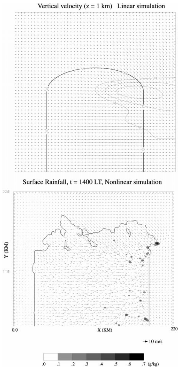
FIG. 17. (a) Surface vectors and vertical velocity at the top of the heat source for linear flow of 4 \text{ m s}^{-1} past a heat source that has only a northern coastline. To be compared with Fig. 1a. (b) Surface vectors and rainwater field for nonlinear flow of 4 \text{ m s}^{-1} past a heat source that has only a northern coastline ( t = 1400 LT). To be compared with Fig. 8d.
