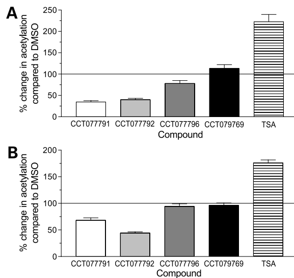
Figure 1. Effect of four isothiazolones on normalized acetylation of HCT116 (A) and HT29 (B) cells following treatment (10 μmol/L) for 24 h. The time-resolved fluorescent cell-based immunosorbent assay was conducted using an acetylated protein antibody. The fluorescent signal obtained in the time-resolved fluorescent cell-based immunosorbent assay was corrected (normalized) by dividing europium counts by the absorbance of the protein concentration. Data are normalized acetylation as a percentage change from DMSO control. Columns , mean of eight replicates for one typical experiment; bars , SD. Cells were also exposed to trichostatin A (TSA; 66 nmol/L) for 24 h in the assay as a positive control. Columns , mean of three replicates; bars , SD.
