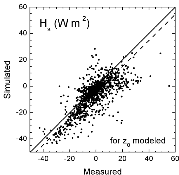
FIG. 7. Hourly averaged eddy-covariance measurements of the sensible heat flux, H_s , and the values simulated with SNTherm with z_0 parameterized as in (3.3). The solid line is 1:1; the dashed line is the best fit, \text{Sim} = 0.989 \text{ Meas} - 4.754 , and r = 0.735 .
