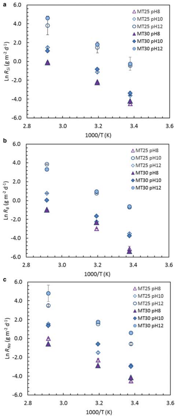
FIG. 2. Ln normalized dissolution rate ( R_i , \text{g m}^{-2} \text{ d}^{-1} ) as a function of the inverse of temperature (from 23 to 70°C) and pH (23°C) of 8.0, 10.0 and 12.0 of: (a) Si; (b) B; and (c) Na, for MT25 and MT30 blend simulated waste glass.
