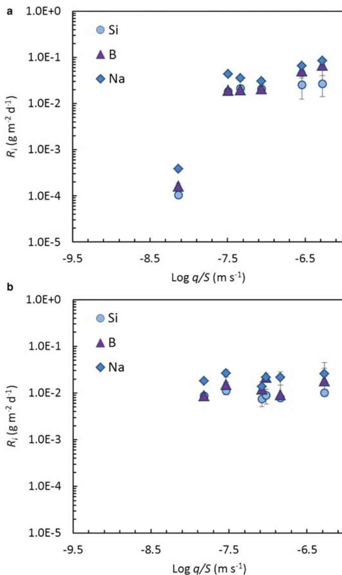
FIG. 1. Normalized dissolution rate ( NR_i , \text{g m}^{-2} \text{d}^{-1} ) as a function of flow rate ( q ) to sample surface area ( S ), ( \text{m s}^{-1} ), for Si, B and Na at T=40^\circ\text{C} and \text{pH}(23^\circ\text{C})=8.0 for (a) MT25 and (b) MT30 blend simulated waste glass.
