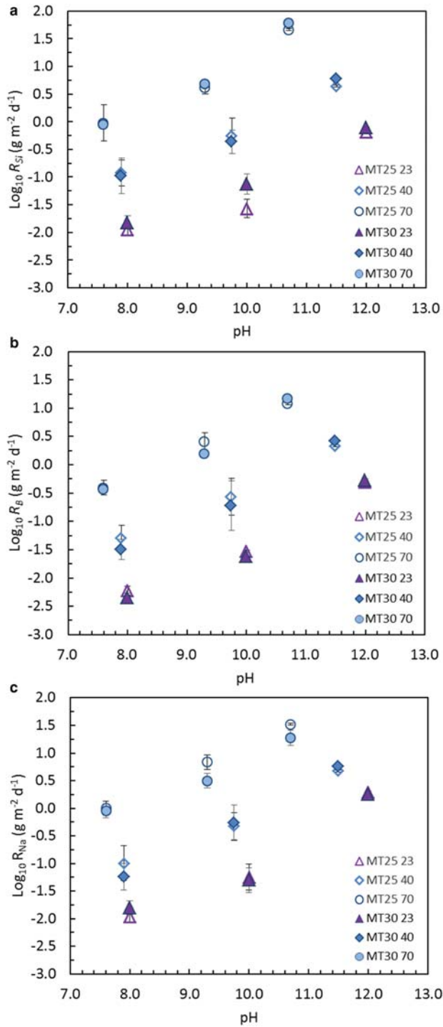
FIG. 3. \text{Log}_{10} normalized dissolution rate ( R_p , \text{g m}^{-2} \text{d}^{-1} ) as a function of temperature- (23, 40 and 70°C) corrected pH for: (a) Si; (b) B; and (c) Na, released from MT25 and MT30 blend simulated waste glasses.
