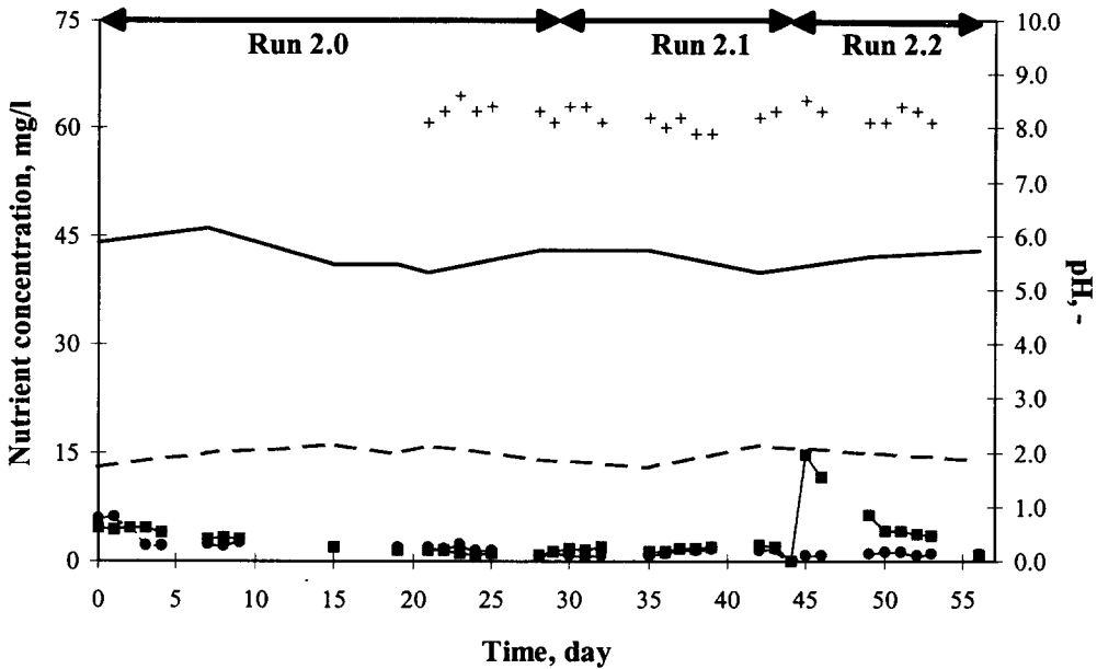
Figure 3. Experimental campaign 2: Height of the Siporax™ packed bed is 200 mm. Average pH and DO concentration in the feed are 7.7 and 6.5 mg/l, respectively. Average DO concentration in the effluent is 2.0 mg/l. — inlet \text{NH}_4^+\text{-N} , - - inlet \text{NO}_3^-\text{-N} , ■ outlet \text{NH}_4^+\text{-N} , ● outlet \text{NO}_3^-\text{-N} , + outlet pH.
