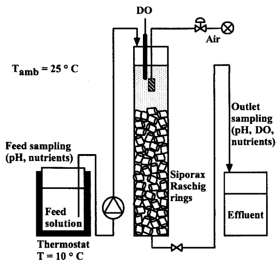
Figure 1. Set-up for the experiments with Siporax™
