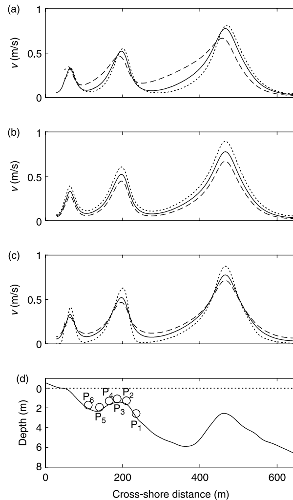
Figure 1 | Alongshore current \bar{v} versus cross-shore distance x showing the effect of changing the wave-front slope \beta , apparent bed roughness k_a and eddy viscosity \nu . In all panels, the offshore conditions are: offshore root-mean-square wave height = 1.5 m, wave period = 8 s and wave angle relative to shore normal = 30°, with no wind and tidal forcing. The solid curve in panels (a)–(c) is the standard run ( \beta = 0.1 , k_a = 0.1 m and \nu = 0.5 m 2 /s). Other curves correspond to changes in one parameter with the others held constant: (a) \beta = 0.15 (dotted line) and \beta = 0.05 (dashed line), (b) k_a = 0.05 m (dotted line) and k_a = 0.2 m (dashed line), (c) \nu = 0 m 2 /s (dotted line) and \nu = 1 m 2 /s (dashed line). (d) The depth profile was measured at Egmond on 15 October 1998. The shallow parts of the profile near cross-shore distances of 200 and 460 m are morphological features known as nearshore sandbars. The circles in (d) are the instrumented positions used in the present work.
