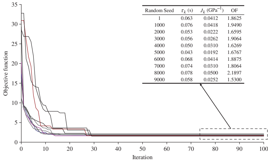
Figure 3 | Variation of the minimum objective function value (OF) for each GA simulation (10 random seeds) and the respective optimal values of the viscoelastic parameters ( \tau_1 and J_1 ).
