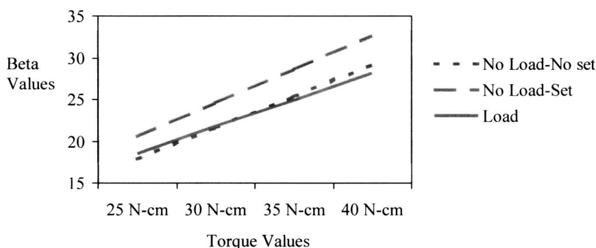
FIGURE 5. Regression lines for all groups.
