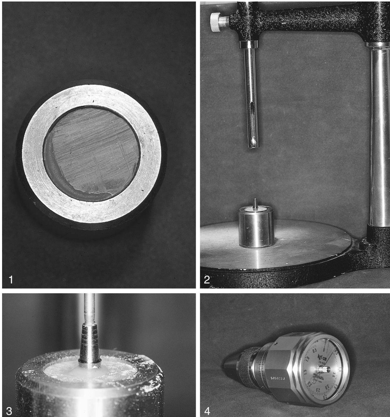
FIGURES 1–4. FIGURE 1. A hollow stainless steel cylinder was filled with autopolymerizing clear resin and allowed to cure for 4 hours at room temperature. FIGURE 2. Each resin cylinder was placed on a surveyor so that the upper surface of the cylinder was perpendicular to the arm of the surveyor. FIGURE 3. The implants were embedded in the clear resin up to the level of the second thread from the implant head. FIGURE 4. Tohnichi torque gauge. (Tohnichi America Corporation, Northbrook, Ill).
