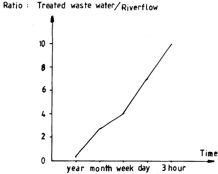
Fig. 4. Ratio between discharge of treated wastewater and the natural river-flow for different time-scales.
