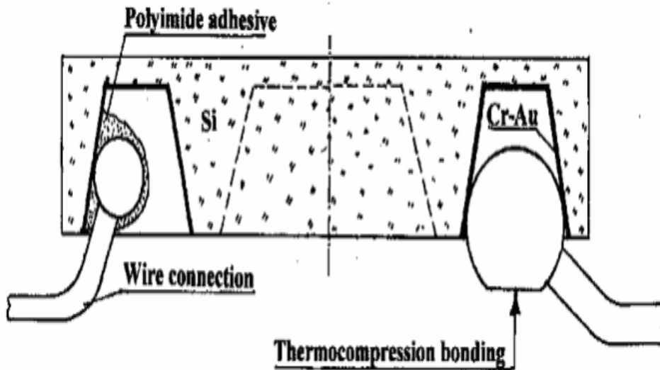
Fig 5. Adhesive and thermocompression bonding of wire connections.
