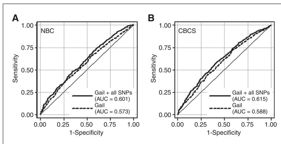
Figure 1. Receiver operating characteristic curves and the area under these curves (AUCs) for the Gail model (dashed line) and the model with the Gail covariates and all 9 study SNPs of Tables 1 and 3 (solid black line). A, NBC study: Gail + all SNPs versus Gail alone; P = 0.026 . B, CBCS study: Gail + all SNPs versus Gail alone; P = 0.003 .
