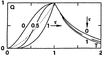
Fig. 5. Hydrographs Q(\bar{T}) for various hystograph shapes, \tau , for which the time of concentration is equal to the precipitation time; (...) uniform precipitation.
