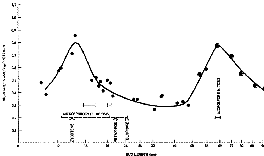
FIG. 2. Soluble sulfhydryl concentration during development of lily anther. The small bars over microsporoctye meiosis indicate the intervals of tapetal cell mitosis (7). Each dot represents the average of values obtained from two groups of anthers. The circled dots are drawn from analyses already published (2).
