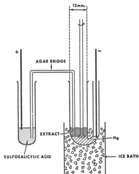
FIG. 1. Arrangement for electrolytic reduction of disulfides. The main cell is made from a test tube cut to appropriate length and fitted with a side arm. The stirrer is flattened at one end to provide adequate agitation. The electrodes are platinum, and the sulfosalicylic acid is a 4 per cent solution.
