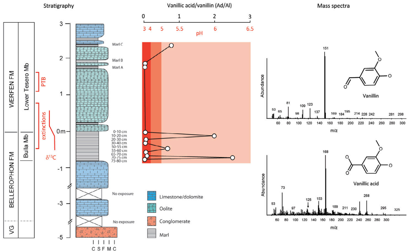
Figure 1. Ratios of vanillic acid to vanillin [acid to aldehyde ratio, (Ad/Al) n ] in latest Permian and earliest Triassic organic matter assemblages from the Vigo Meano section (southern Alps, Italy), providing proxy evidence for pulses of soil acidification (pH <4). For calibration of (Ad/Al) n values to pH values, see the Data Repository (Fig. DR1 [see footnote 1]). VG—Val Gardena Formation; PTB—approximate position of the Permian-Triassic boundary; extinctions—interval of principal marine extinction and floral turnover in southern Alps; \delta^{13}\text{C} —position of end-Permian negative carbon-isotope shift in southern Alps. Letters at bottom of stratigraphic column, from left to right, correspond to clay, silt, fine sand, medium sand, and coarse sand, respectively.
