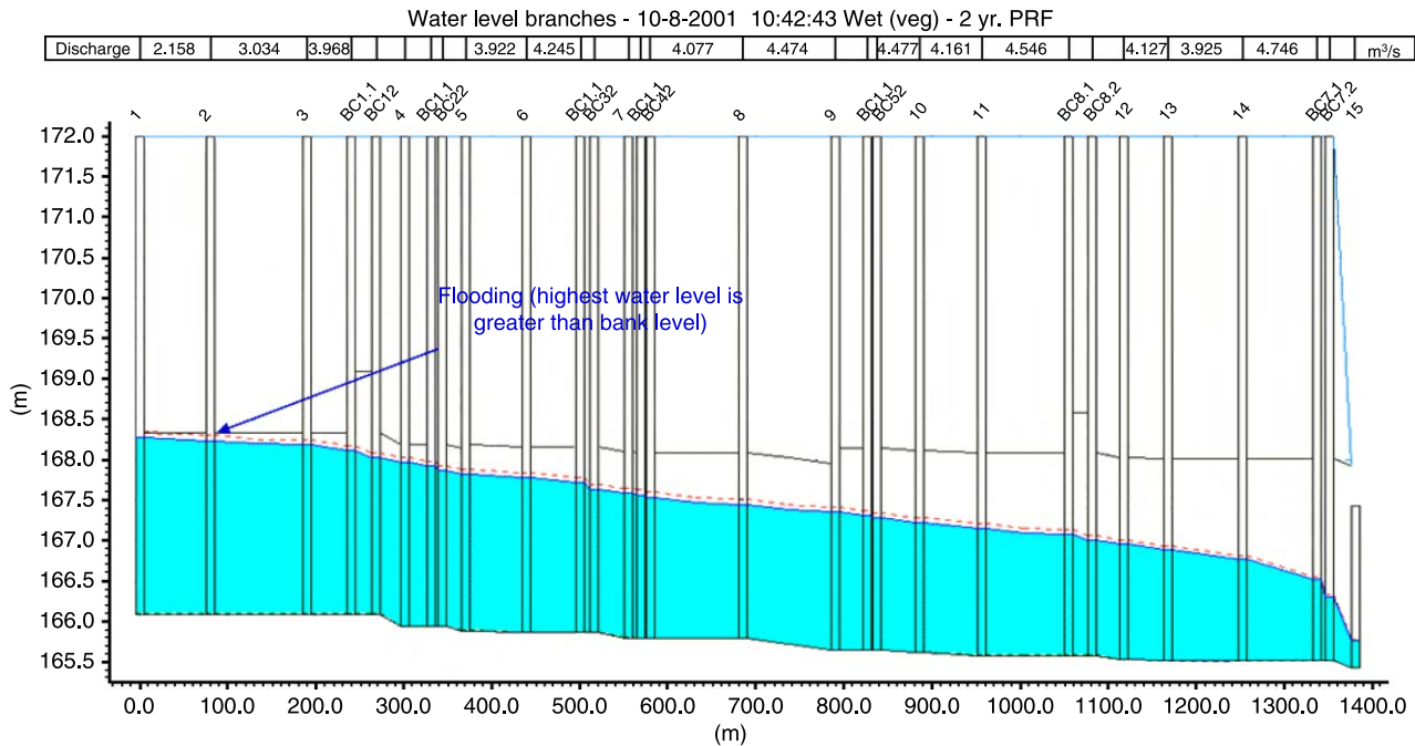
Figure 6 | Water level along the Nam Pasak II channel for a 2yr return period rainfall in vegetated condition Case 2.
