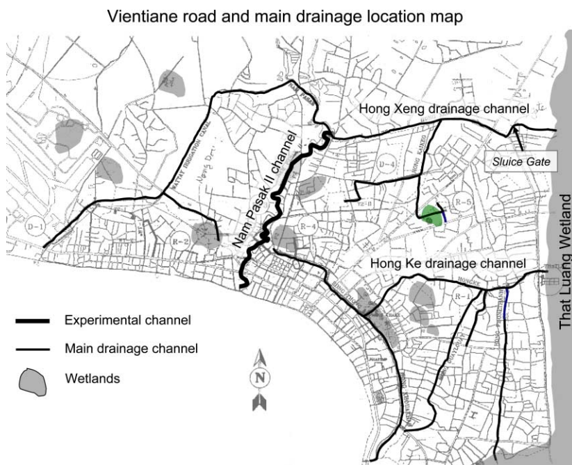
Figure 3 | Locations of the Nam Pasak II channel (study site) and other major drainage channels and wetlands in Vientiane.
