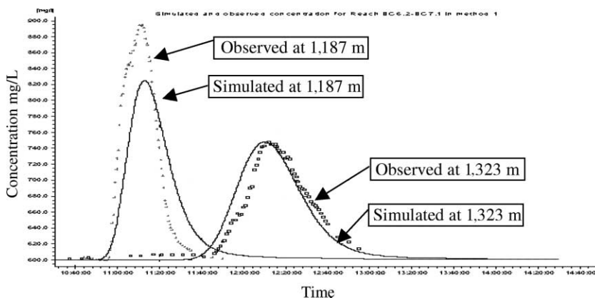
Figure 5 | Calibration plot for the downstream reach (1.05–1.35 km) of the Nam Pasak II experimental channel.
