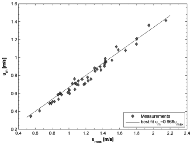
Figure 2 | Relation between mean and maximum velocities at the gauged river section of Pontelagoscuro.
