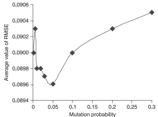
Figure 5 | Performance of uniform mutation.
