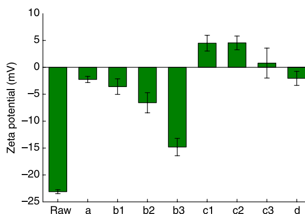
Figure 5 | Zeta potentials of sludge developed from synthetic raw water containing various types and concentrations of organic materials.
