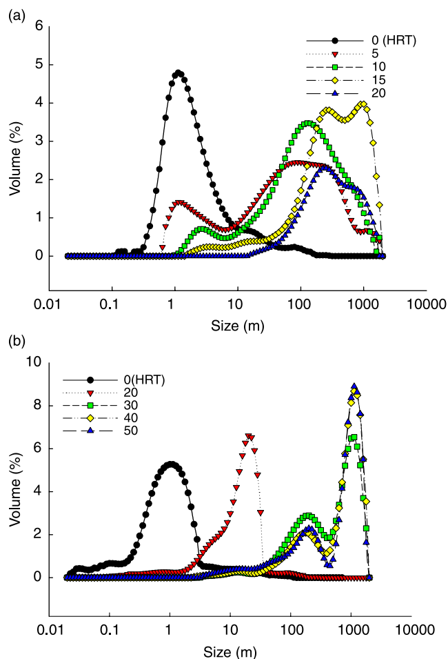
Figure 4 | Size distribution of flocs in (a) humic acid-laden blanket sludge (b2); (b) salicylic acid-laden blanket sludge (c2).
