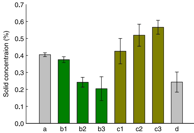
Figure 2 | Effect of type and concentration of organic compounds on solid concentration of sludge blanket.
