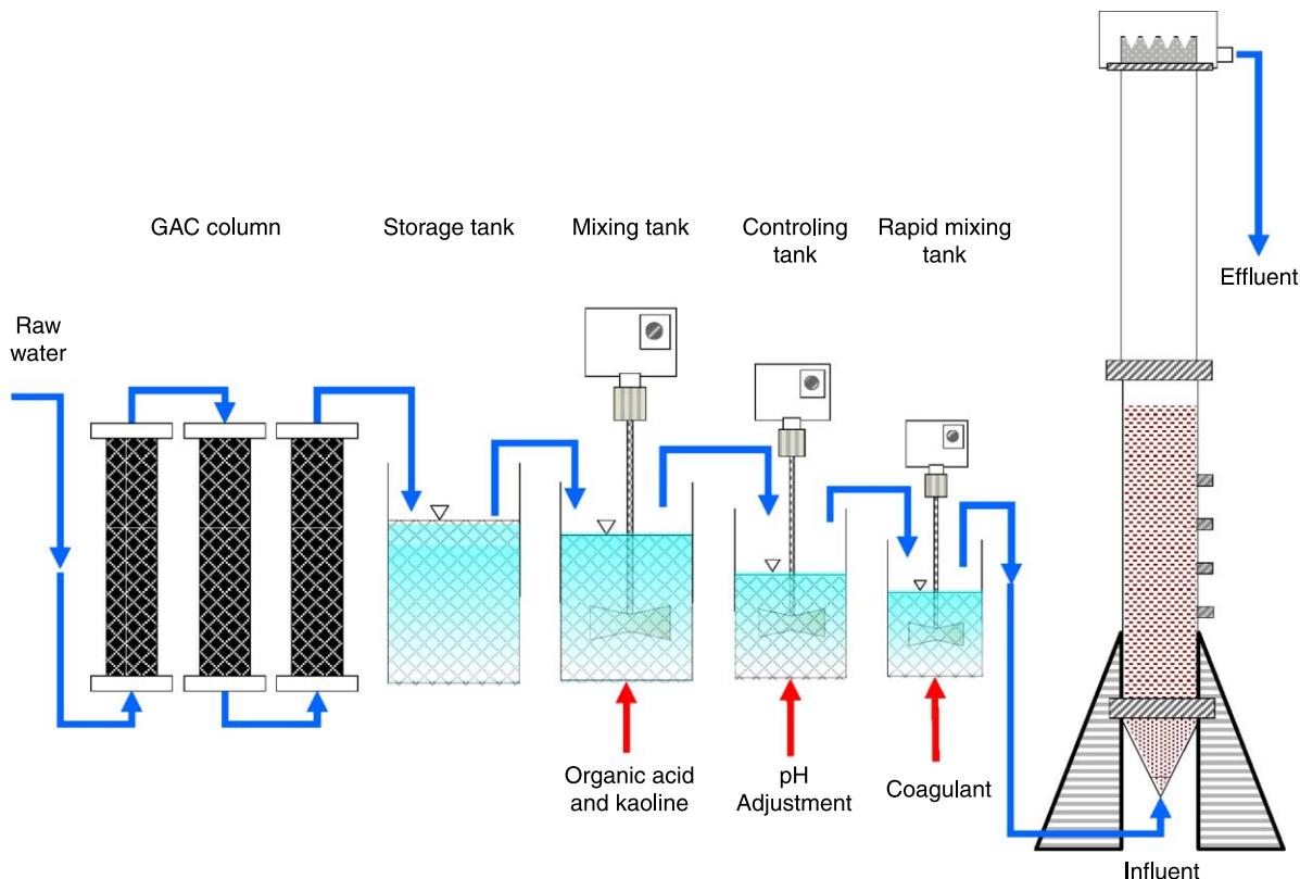
Figure 1 | Schematic diagram of the water clarifier module containing GAC column, storage tank, chemical mixing tank, pH controlling tank, coagulation tank and SBC.
