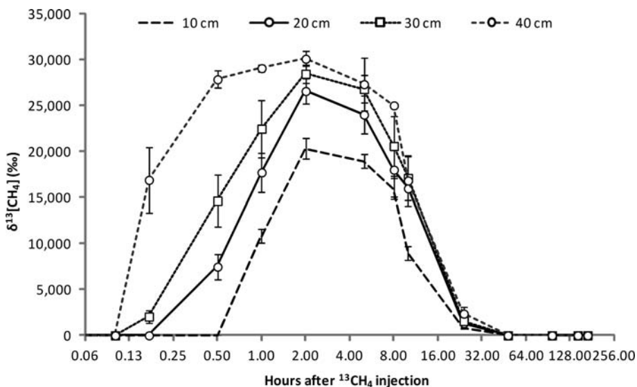
FIG. 7. Laboratory results. Average \delta^{13}\text{CCH}_4 measured within gas samples obtained from four depths in LE 4. Figure published with the permission of the NDA.
