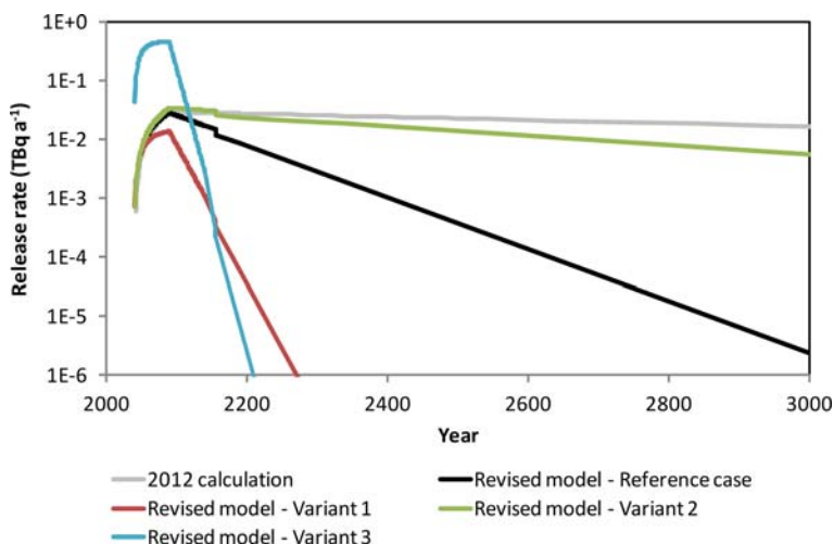
FIG. 5. Results from the revised model for the release of carbon-14 from graphite. Figure published with permission of the NDA.
