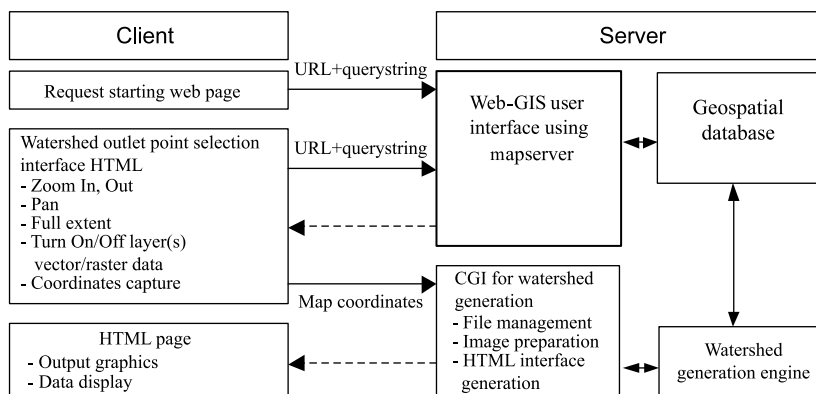
Figure 2 | Schematic diagram for the description of procedures in watershed delineation system operation.
