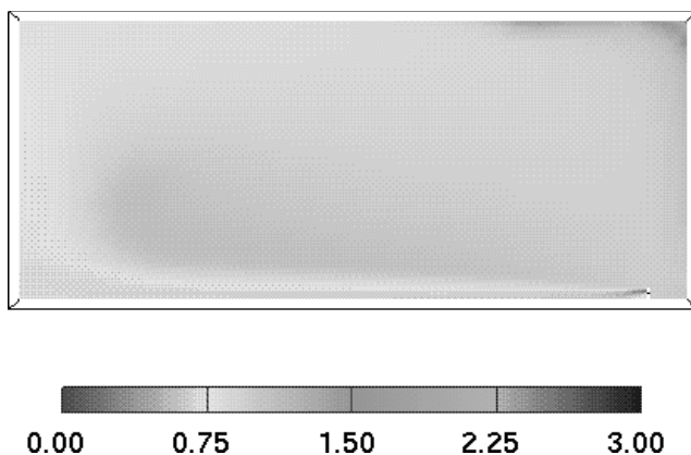
Figure 3 | Water age distribution inside a tank.
