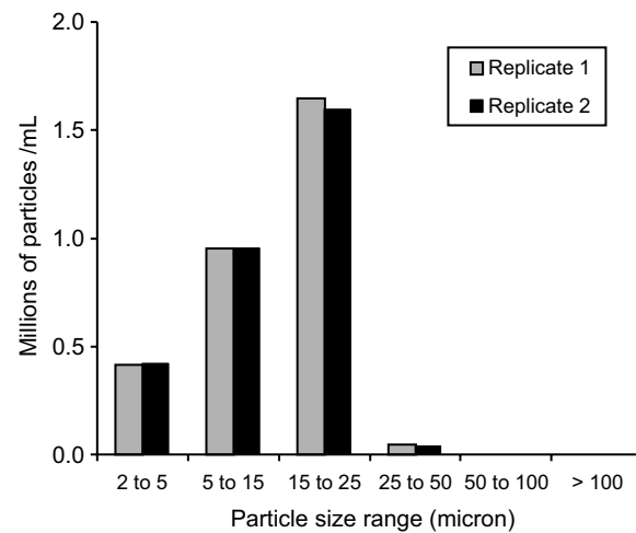
Figure 3 | Particle size distribution of the suspended particulate matter concentrated from Lake Okanagan, BC (before dilution and parasite addition). The distribution does not include the contribution of the prepared parasites.
