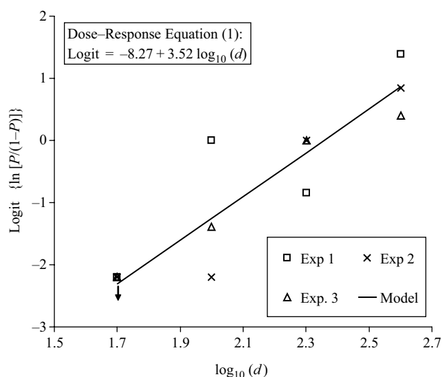
Figure 1 | Results of three dose–response experiments for the C. parvum oocyst batch used in UV exposure experiments, and the computed dose–response model. Note: each datum represents infectivity determined in 10 mice. The arrow indicates that the result for one of the three experiments conducted at the dose of 50 oocysts per mouse was below detection (no mice were positive for infection).
