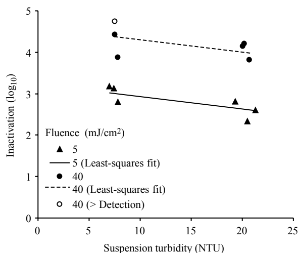
Figure 6 | Inactivation ( -\log_{10}d/d_0 ) of Giardia muris oocysts in UV exposure experiments as a function of turbidity.
