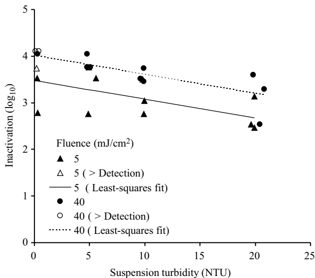
Figure 7 | Inactivation ( -\log_{10}d/d_0 ) of Cryptosporidium parvum oocysts in UV exposure experiments as a function of suspension turbidity.
