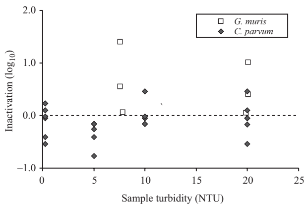
Figure 5 | Inactivation ( -\log_{10}d/d_0 ) of Giardia muris cysts and Cryptosporidium parvum oocysts in non-UV-exposed positive control experiments as a function of suspension turbidity.
