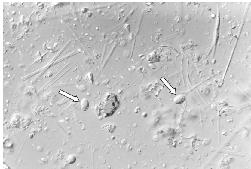
Figure 4 | Photograph of a 20 NTU suspension of prepared Giardia muris cysts and suspended particulate matter viewed on a hemacytometer slide under 400\times light microscopy after concentration by centrifugation. (The arrows indicate putative Giardia muris cysts.)
