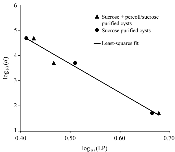
Figure 2 | Results of dose–response experiments in adult male C3H/HeN mice with G. muris cysts. (LP = latent period of infection in days as defined by Equation (2)).
