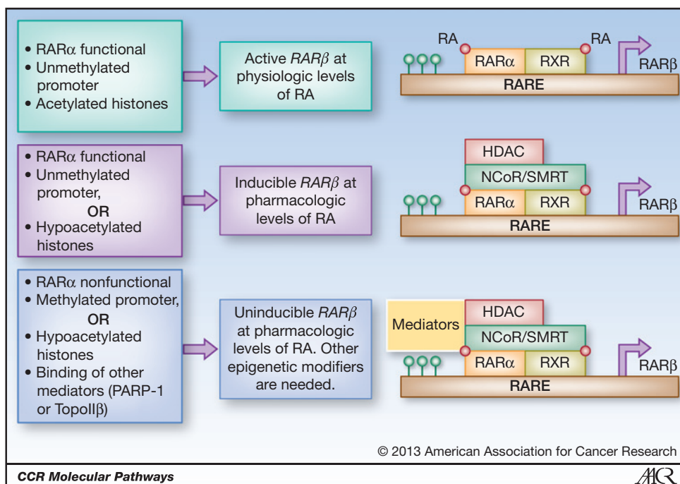
Figure 2. Mechanism of activation of RARβ , an important downstream effector of the RA pathway, in cancer growth inhibition. Under conditions where RARα is functional and the RARβ promoter is not epigenetically silenced, physiologic levels of RA can activate RARβ expression. A small number of solid tumors display this phenotype. Under less ideal conditions in which the RARβ promoter is hypoacetylated, pharmacologic doses of RA are needed to activate RARβ . In the majority of solid tumor types, the RARβ promoter is methylated and/or the histones are significantly deacetylated. In this case, treatment with pharmacologic doses of RA is not sufficient to overcome the repressive effect of epigenetic silencing. Epigenetic-modifying drugs such as DNA methyltransferases or HDAC inhibitors are needed to release the epigenetic stress and activate the RARβ gene. NCoR, nuclear receptor corepressor 1; SMRT, silencing mediator for retinoid and thyroid receptors.
