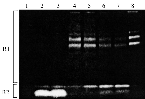
Fig. 4 SDS-PAGE analysis (5% nonreducing gel) of A-431 cell lysates prepared from time-coursed incubations with free BPD or BPD-C225 PIC. The photosensitizer fluorescence of the gel was imaged as described in Materials and Methods. Cell lysates were prepared by incubating cells for various times at 37°C with 280 nmol/L BPD content of free BPD or PIC (7 BPD/antibody). Intact PIC runs in region R1, and broken down PIC or free BPD runs in region R2. (Lane 1) cells incubated with media only, (lane 2) cells incubated for 1 hour with free BPD, (lane 3) cells incubated for 40 hours with free BPD, (lane 4) cells incubated for 1 hour with PIC, (lane 5) cells incubated for 4 hours with PIC, (lane 6) cells incubated for 17 hours with PIC, (lane 7) cells incubated for 40 hours with PIC, and (lane 8) 0.5 \mu\text{L} of the original 30 \mu\text{mol/L} (BPD content) stock solution of PIC.
