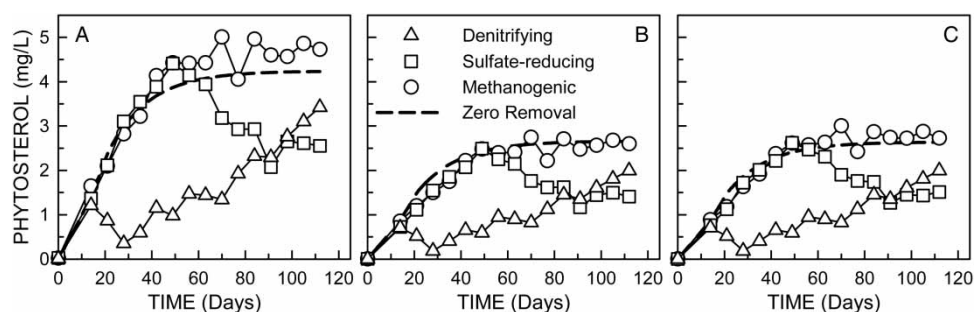
Figure 2 | Phytosterol profiles in the three semi-continuously fed cultures. A, \beta -sitosterol; B, stigmasterol; C, campesterol (broken lines represent phytosterol concentrations calculated taking into account wasting and feeding of the cultures and assuming complete recalcitrance of the three phytosterols).
