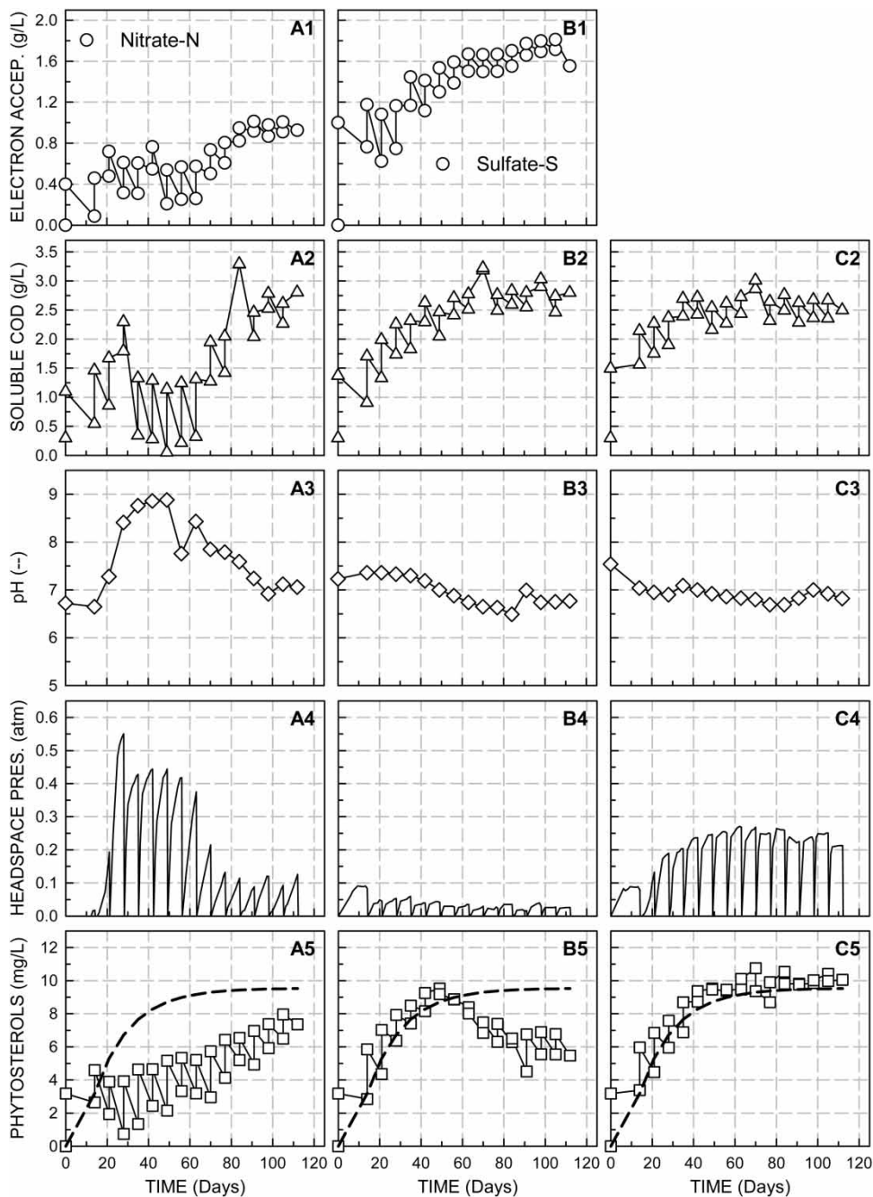
Figure 1 | Time course of (1) electron acceptor (i.e. nitrate or sulfate), (2) soluble COD, (3) pH, (4) headspace pressure, and (5) total phytosterols in semi-continuously fed nitrate-reducing (A), sulfate-reducing (B), and methanogenic (C) cultures (broken lines represent phytosterol concentrations calculated taking into account wasting and feeding of the cultures and assuming complete recalcitrance of the three phytosterols).
