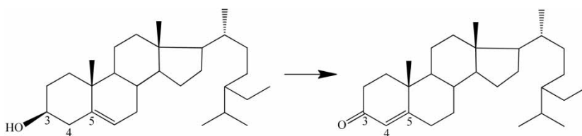
Figure 3 | Production of stigmast-4-en-3-one from \beta -sitosterol.
