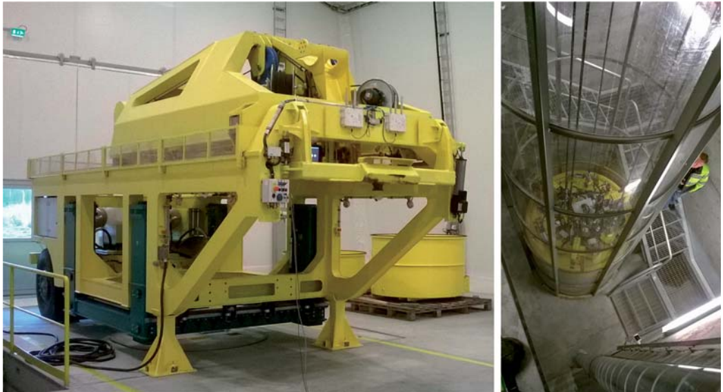
FIG. 5. Left image: the buffer installation machine in the test hall during the lifting test. Testing is done with a concrete block. Right image: the vertical deposition hole, a concrete test block is being lowered to the bottom.
