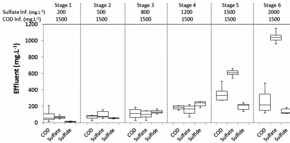
Figure 3 | Boxplot analysis of organic matter removal (COD), sulfate reduction and sulfide concentration.
