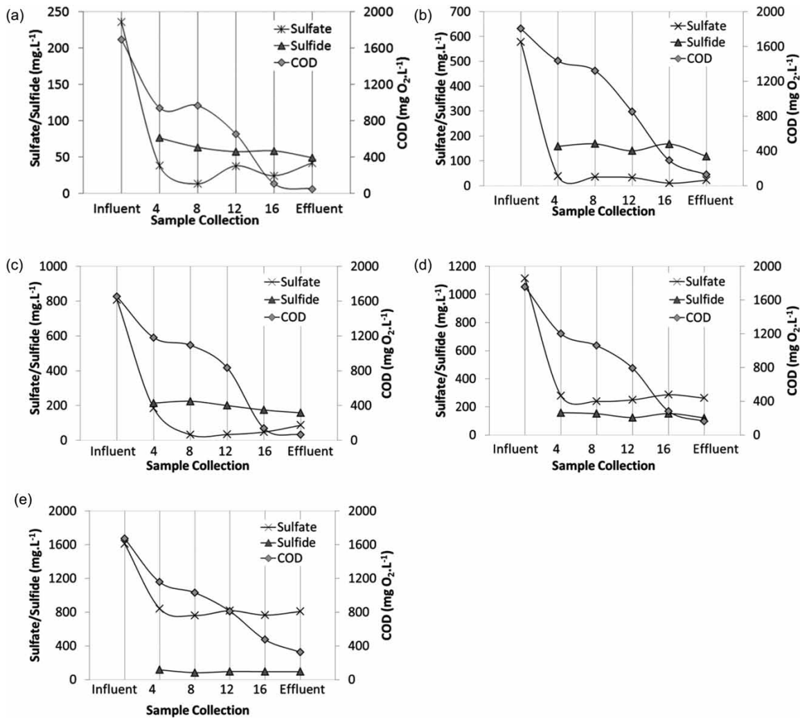
Figure 4 | Reactor concentration gradients: (a) stage 2 – sulfate concentration = 200 mg L -1 ; (b) stage 3 – sulfate concentration = 500 mg L -1 ; (c) stage 4 – sulfate concentration = 800 mg L -1 ; (d) stage 5 – sulfate concentration = 1,500 mg L -1 ; (e) stage 6 – sulfate concentration = 2,000 mg L -1 .
