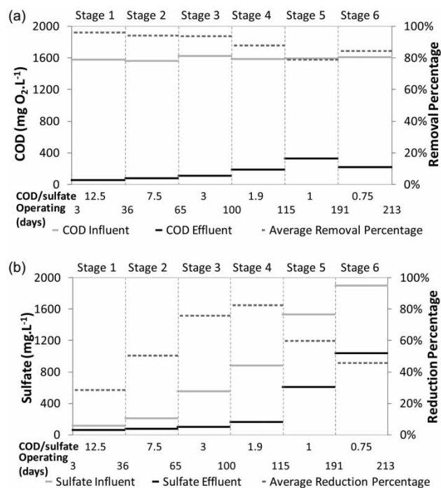
Figure 2 | (a) Average quantity of COD removed; (b) average quantity of sulfate reduction.
