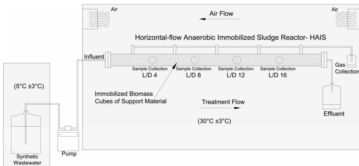
Figure 1 | Scheme of the bench-scale HAIS reactor.
