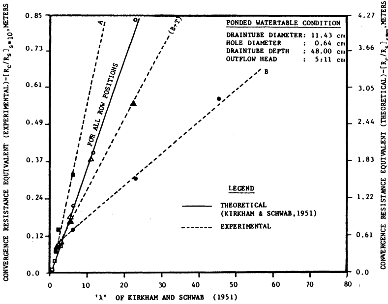
Fig. 4. Comparison of experimental and theoretical convergence resistance equivalent. \lambda of Kirkham and Schwab (1951).
