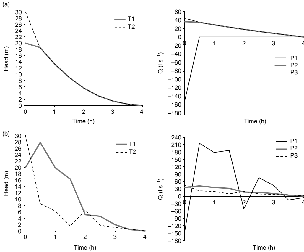
Figure 6 | As for Figure 2 with Δt = 30 min. (a) the disappearance of the surge in tank 1 is due to the coarse time discretization. (b) Note the large errors in the flow of pipe 1 and in the water level oscillations of both tanks.
