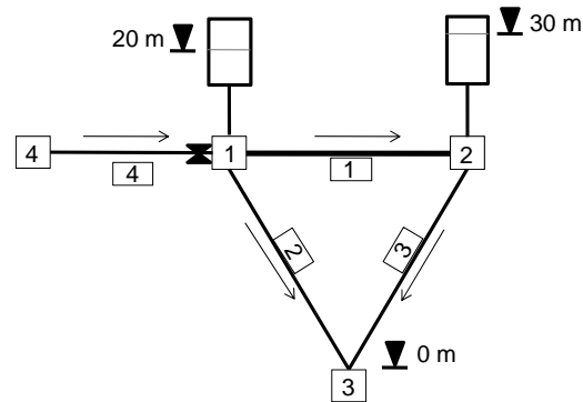
Figure A1 | Schematic representation of the example to be run using EPANET 2. A null demand junction node 4 and a closed pipe 4 were added to the original scheme without modifying the expected system behaviour.
