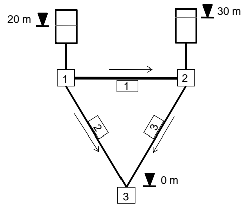
Figure 1 | Schematic representation of the first example. Two emptying interconnected tanks starting at time zero with different water levels.
