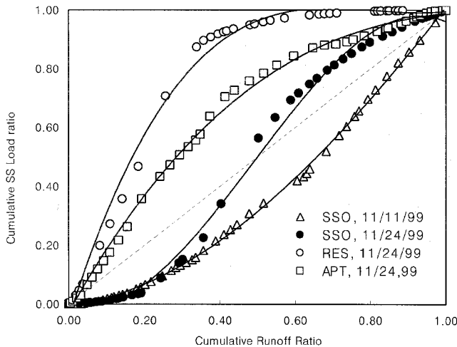
Figure 5 Polynomial equation curves and observed first flush for SS
