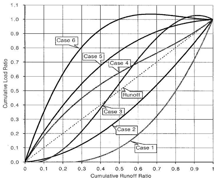
Figure 6 Shape of first flush curves with polynomial equation constants
