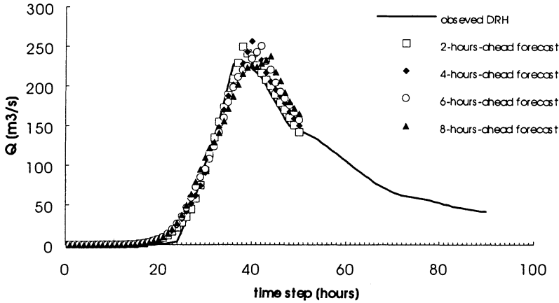
Fig. 7. Observed direct runoff hydrograph and 2-4-6-8 hours ahead forecasts by means of Extended Kalman Filter procedure for the May 1977 event. The value of \sigma was assumed to be 270 mm and initial condition C^*_0 to be 65 mm.
