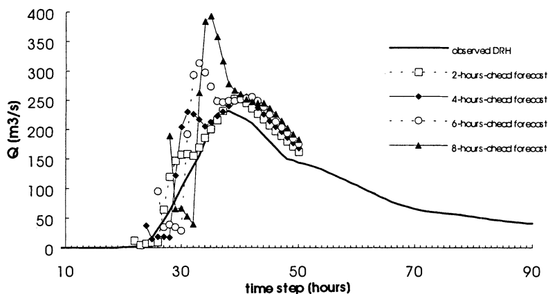
Fig. 5. Observed direct runoff hydrograph and 2-4-6-8 hours ahead forecasts by means of the on-line optimization of parameters \sigma and C^*_0 for the May 1977 event.
