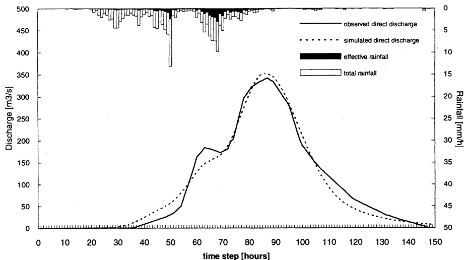
Fig. 2. Observed and simulated direct discharge after the off-line automatic calibration for the November 1941 event (estimated values: \sigma = 362 mm, C^*_0 = 83 mm).
