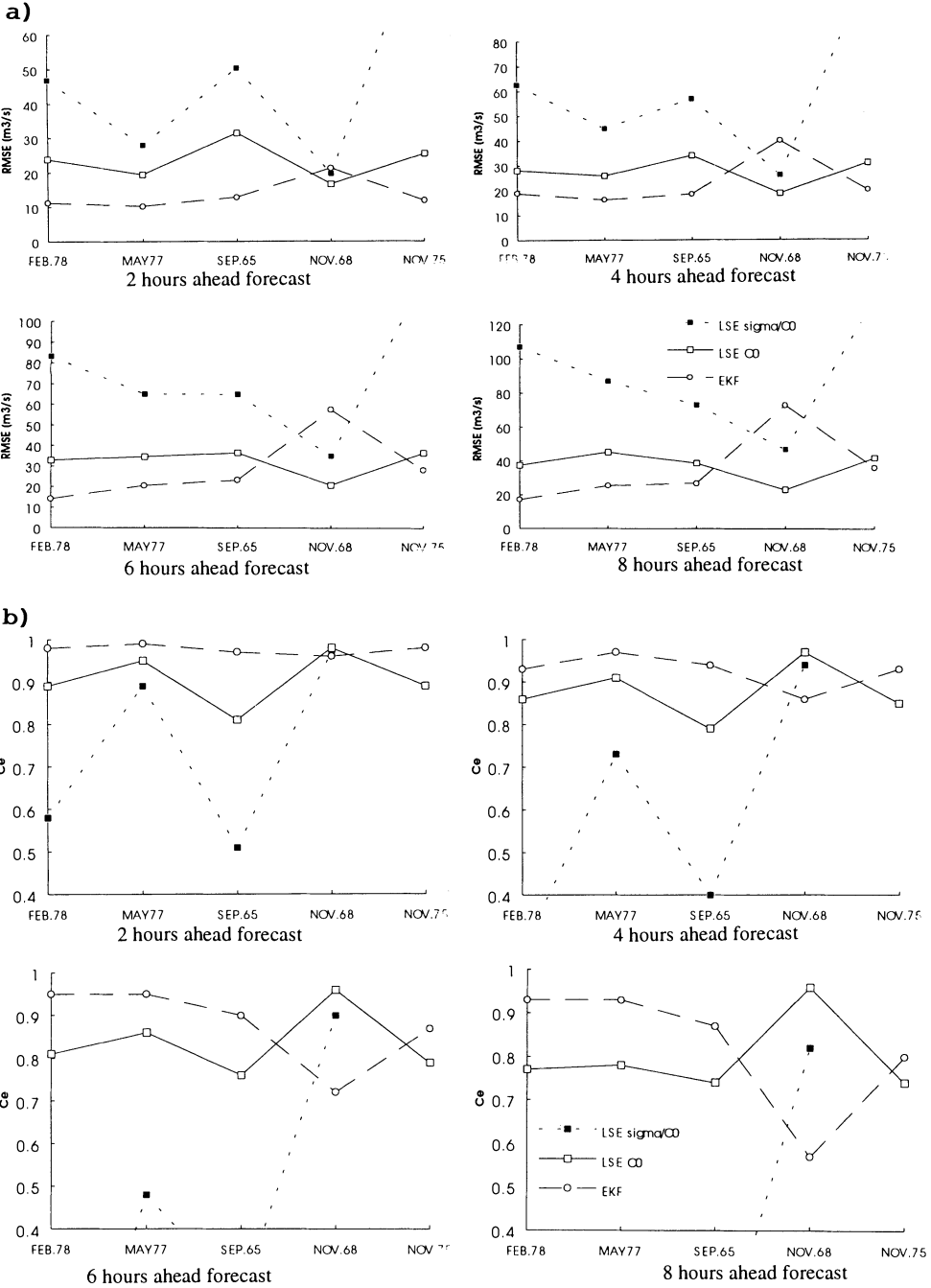
Fig. 3. Comparison of the performances in forecast for the three methods in terms of root mean square errors (RMSE) and coefficient of efficiency ( C_e ).
