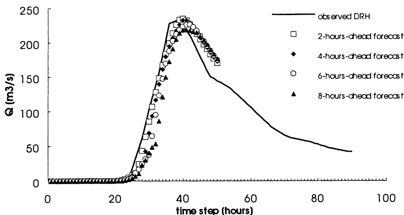
Fig. 6. Observed direct runoff hydrograph and 2-4-6-8 hours ahead forecasts by means of the on-line optimization of the initial condition C^*_0 for the May 1977 event (the value of \sigma was assumed to be 270 mm).
