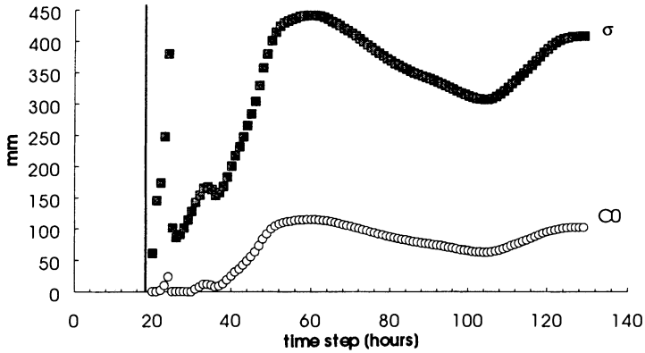
Fig. 4. Fluctuations of estimated values of \sigma and C^*_0 in the course of the adaptive calibration procedure for the May 1977 event.
