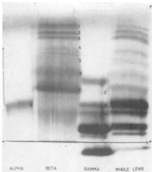
Fig. 3. Starch-gel electrophoretic separation of alpha, beta, and gamma crystallin fractions of the rabbit lens, isolated by the methods of Spector 12 and run in the same gel as a whole lens homogenate. Protein concentrations: alpha, 40 mg. per milliliter; beta, 140 mg. per milliliter; gamma, 80 mg. per milliliter; whole lens, 140 mg. per milliliter. Labels are as in Fig. 1.
