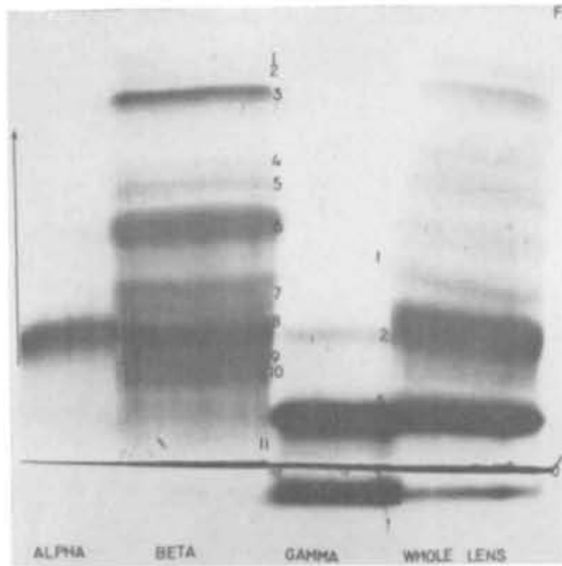
Fig. 5. Alpha, beta, and gamma crystallin fractions from 40 pooled rat lenses, prepared by the methods of Spector, 12 run in the same gel as a whole rat lens homogenate. Protein concentrations: alpha, 40 mg. per milliliter; beta, 137 mg. per milliliter; gamma, 90 mg. per milliliter; whole lens, 140 mg. per milliliter. Note that beta and gamma proteins are present in relatively greater concentrations than in whole lens homogenates.
