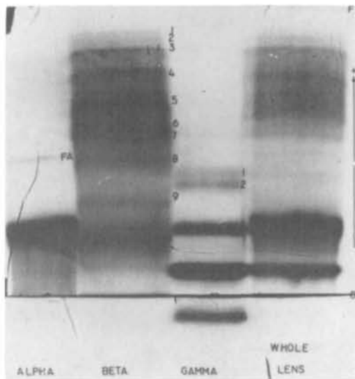
Fig. 1. Starch-gel electrophoretic patterns produced by calf alpha, beta, and gamma crystallin fractions isolated by the precipitation and gel-filtration methods of Spector. 12 Protein zones arising from each fraction are numbered in order of decreasing mobility in starch-gel electrophoresis. Protein concentrations: alpha, 40 mg. per milliliter; beta, 140 mg. per milliliter; gamma, 90 mg. per milliliter; whole lens, 140 mg. per milliliter. FA , "fast-alpha" zone; F , buffer front; O , sample insertion slot. The concentrations of beta and gamma fractions are relatively greater than in the whole lens homogenates in order to demonstrate the presence of faint zones, such as gamma-1 and gamma-2.
