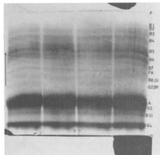
Fig. 2. Starch-gel electrophoresis of calf lens protein homogenates. The arrow indicates the direction of migration from cathode to anode. Lens homogenates from 4 different lenses run in the same gel. Protein zones are labeled according to the fraction of origin and in order of decreasing mobility: O , sample insertion slot; F , buffer front; A , alpha; B , beta; G , gamma; FA , "fast-alpha" protein. Protein concentrations, 135 mg. per milliliter.
