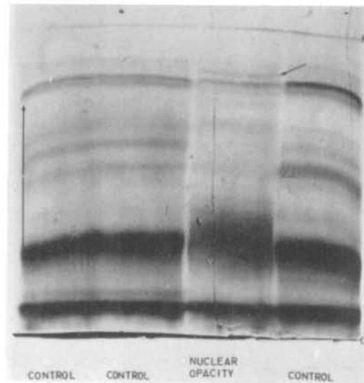
Fig. 8. Electrophoretic pattern produced by a lens bearing a dense nuclear opacity. Note the decreased staining intensity of most beta and gamma zones, the broadening of the alpha zone, and the apparently new beta zone (arrow). Protein concentrations, 110 mg. per milliliter.
