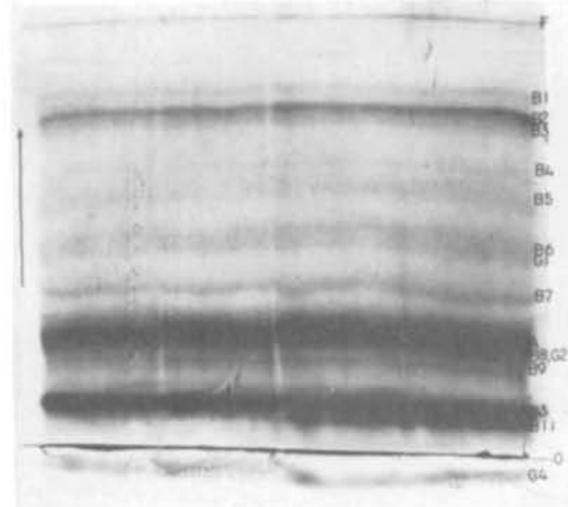
Fig. 6. Separation of normal rat lens soluble proteins. Four lenses from 2 rats. Protein concentrations are 130 mg. per milliliter. Labels as in Fig. 1.
