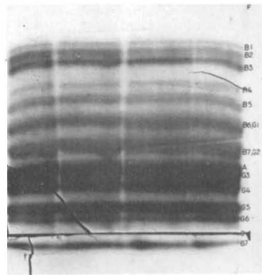
Fig. 4. Four normal rabbit lenses separated by starch gel electrophoresis. Protein concentrations, 145 mg. per milliliter. Labels as in Fig. 2.
