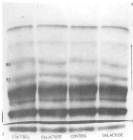
Fig. 7. Patterns produced by lens homogenates from the 2 lenses of a normal rat and a rat fed a 50 per cent galactose diet for 24 hours prior to death. Note the changes in beta zones 6 and 7 induced by galactose feeding relative to the control patterns. Protein concentrations, 140 mg. per milliliter. (See text for discussion.)
