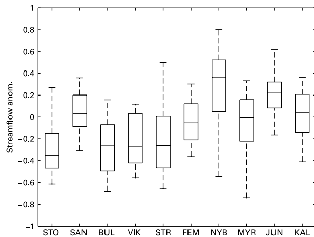
Figure 6 | The spread among the 12 ensemble members for the ten streamflow stations (see station abbreviation in Figure 5) for year 1968. The spread is given in boxplots, in which the median, lower and upper quartiles and minimum and maximum values are given (Patrik Nilsson).
