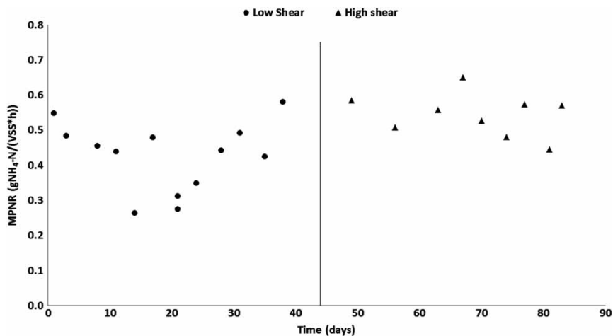
Figure 3 | MPNR when testing shear from GBB MFU (test a). MPNR is normalized to 15^\circ\text{C} .
