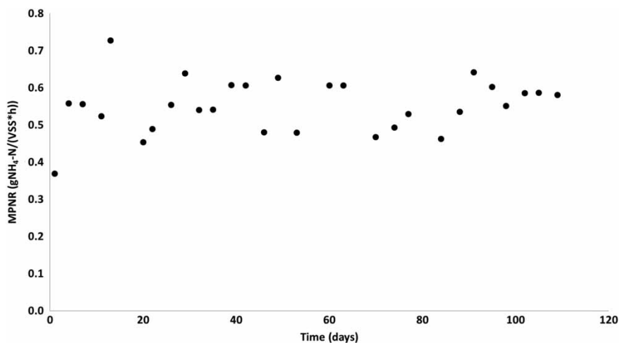
Figure 7 | MPNR when testing selection from the GBB MFU (test c). MPNR is normalized at 15 °C.
