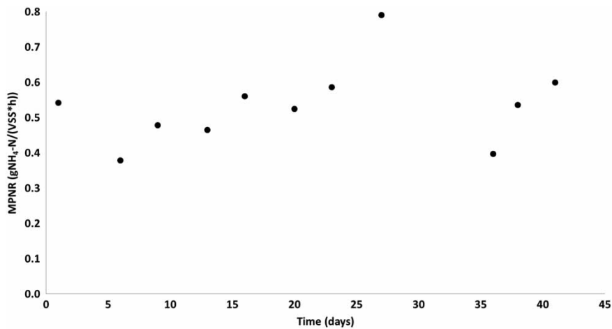
Figure 6 | MPNR when testing shear from the pressure reduction component (test b). MPNR is normalized at 15 °C.
