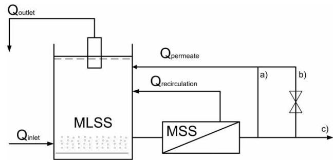
Figure 1 | Overview of test setup to expose activated sludge to shear from GBB membranes (test a) and the pressure reduction component (test b). MSS: membrane suspended solids.
