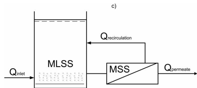
Figure 2 | Overview of test setup to expose activated sludge to selection from GBB membranes (test c).
