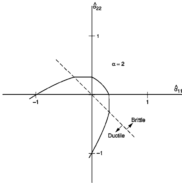
Fig. 1 Biaxial stress state
