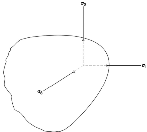
Fig. 4 Yield/failure paraboloid
