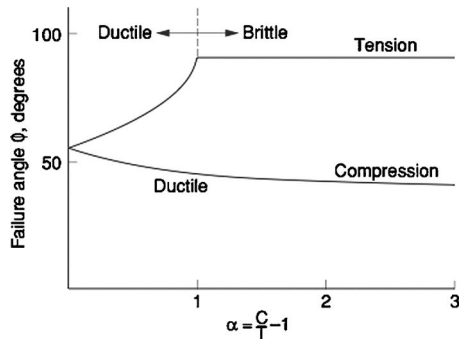
Fig. 7 Failure angles, uniaxial tension and compression
