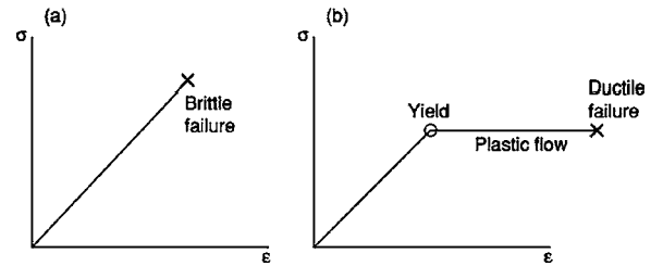
Fig. 2 Brittle failure and ductile yield/failure
