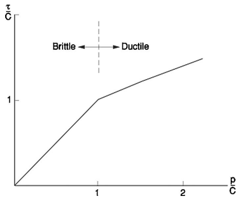
Fig. 5 Shear stress superimposed upon pressure, \alpha = \infty limit, Eq. (12)
