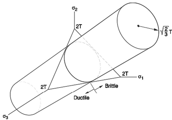
Fig. 3 Mises material, \alpha=0 , ductile yield and brittle failure regions
