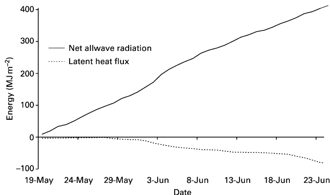
Figure 6 Cumulative net radiation and APM estimated latent heat fluxes over the investigation period
