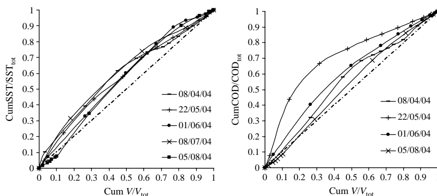
Figure 2 M(V) curves for TSS and COD in runoff resulting from the gas station
