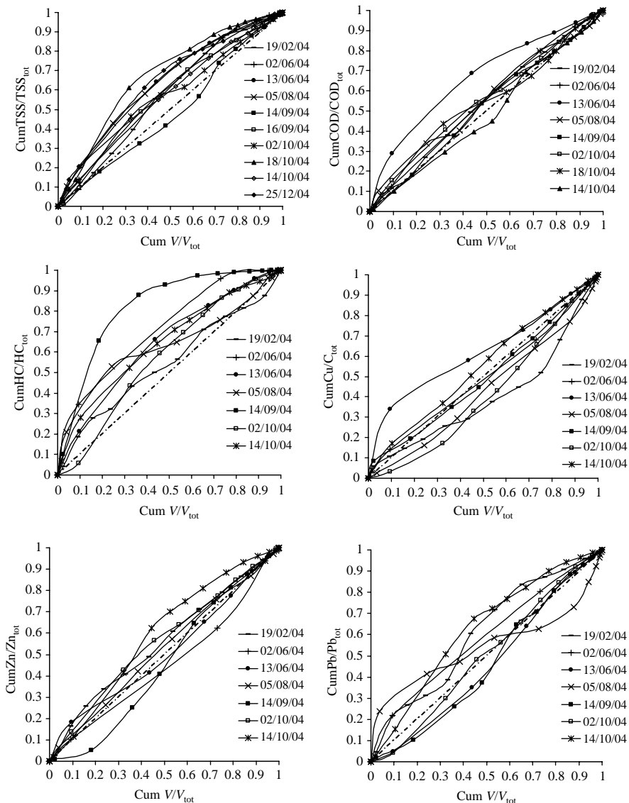
Figure 1 M(V) curves for TSS, COD, total hydrocarbons and heavy metals in dissolved form in runoff resulting from the auto dismantler facility
