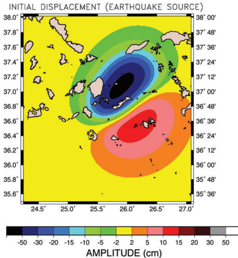
Figure 7. Field of static displacement created by the seismic source inverted in Section 3, obtained using the algorithm of Mansinha & Smylie (1971). These values are used as the initial condition of the hydrodynamic solution under the earthquake scenario.
