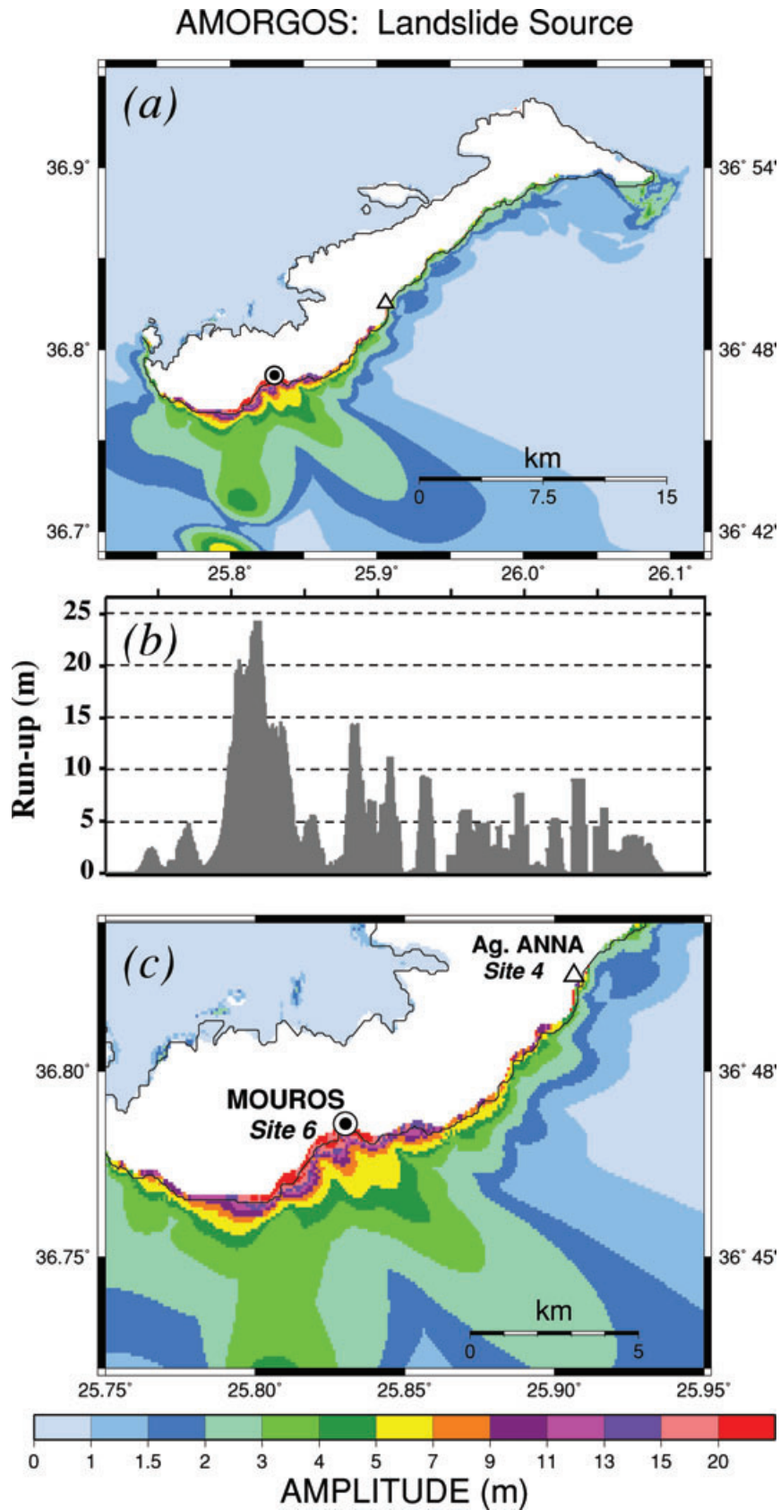
Figure 14. (a) Same as Fig. 10a, under the Amorgos landslide scenario. (b) Simulated runup along the southern coast of Amorgos, plotted as a function of longitude using the same scale as in (a). (c) Close-up of (a) in the vicinity of Sites 4 and 6.
