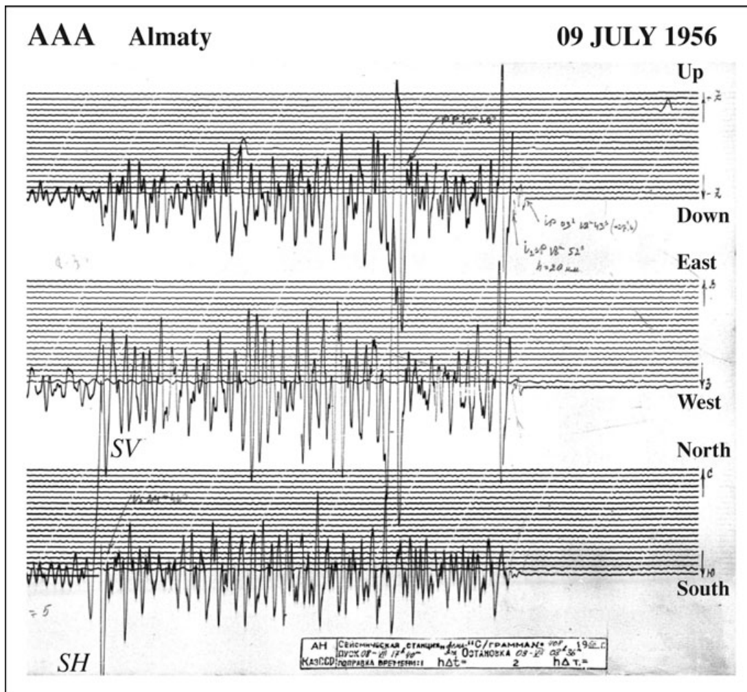
Figure 6. Close-up of 3-D record at Almaty, Kazakstan (AAA). Time increases to the left. For this naturally polarized station (backazimuth \beta = 278^\circ ), we clearly observe a dilatational P wave and SH/SV > 1 .
