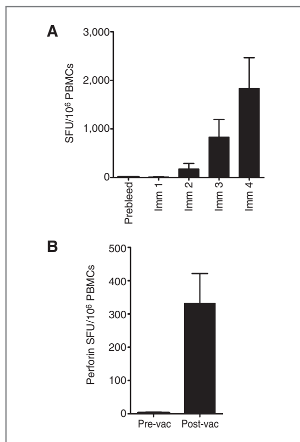
Figure 3. pH 1 TERT elicited robust CTLs in rhesus macaques. A , total IFN- \gamma responses induced by pH 1 TERT following each immunization. Four rhesus macaques were vaccinated with pH 1 TERT, four times intramuscularly followed by electroporation, 6 weeks apart, at 2 mg DNA/each immunization. PBMCs were isolated and stimulated with hTERT peptides for 24 hours. Frequencies of hTERT-specific IFN- \gamma -secreting cells/10 6 PBMCs were determined by IFN- \gamma ELISpot assay. B , enhanced perforin release in immunized monkeys. Prebleed and PBMCs after last immunization were stimulated with hTERT peptides for 24 hours. Frequencies of hTERT-specific perforin-secreting cells/10 6 PBMCs were determined by perforin ELISpot assay. Results are presented as mean \pm SEM.
