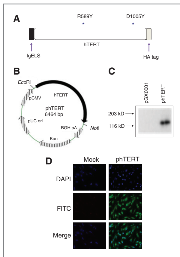
Figure 1. Design and expression of hTERT DNA vaccine. A, schematic of hTERT antigen. The * denotes the incorporated point mutation. B, map of phTERT. C, detection of phTERT expression by in vitro translation. The gene product was immunoprecipitated using an anti-HA (hemagglutinin) tag monoclonal antibody, visualized by SDS-PAGE and autoradiography. D, immunofluorescence assay of phTERT. Transfected rhabdomyosarcoma cells expressing hTERT protein showed typical FITC-fluorescence using a commercial hTERT (C-term) monoclonal antibody. DAPI, 4',6-diamidino-2-phenylindole.
