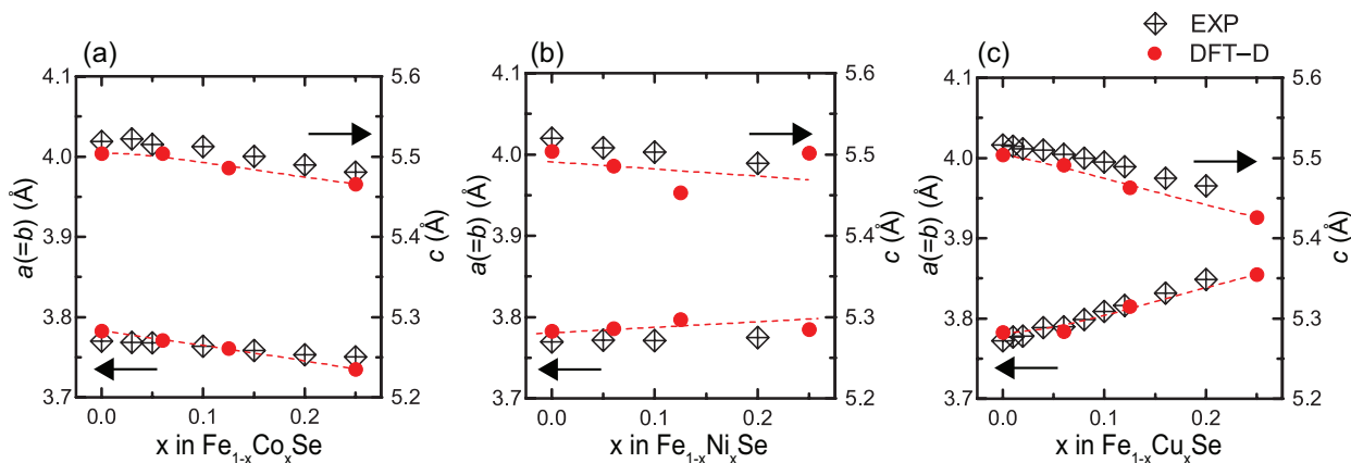
FIGURE 4. Lattice parameters of (a) \text{Fe}_{1-x}\text{Co}_x\text{Se} , (b) \text{Fe}_{1-x}\text{Ni}_x\text{Se} , and (c) \text{Fe}_{1-x}\text{Cu}_x\text{Se} vs. metal mole fraction ( x ). Dashed curves show the trends of calculated data using DFT-D. Experimental data (EXP) are from Thomas et al. (2009) in a, Mizuguchi et al. (2009) in b, and Willams et al. (2009) in c.
