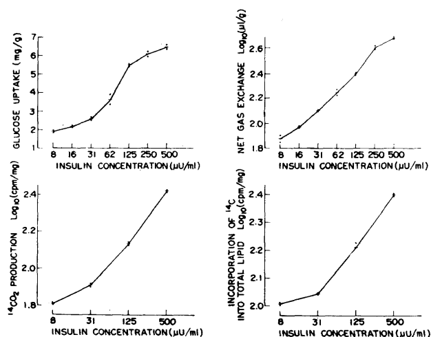
FIG. 2. Four different insulin dose-response curves by different parameters of fat pad metabolism. Parameters are glucose uptake, net gas exchange, C-14-O 2 production from D-glucose-U-C-14, and incorporation of C-14 into total lipid, respectively. The shapes of these four curves were relatively similar to each other over the same range of insulin doses.
