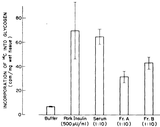
FIG. 3. Incorporation of C-14 into glycogen of rat epididymal adipose tissue from D-glucose-U-C-14 in vitro. Each bar represents the mean and standard error of three experiments. Insulin, Fractions A and B all stimulated C-14 incorporation into fat pad glycogen.
