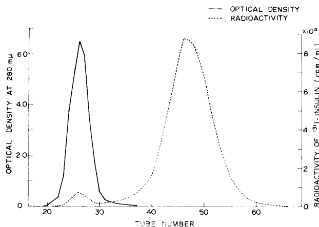
FIG. 1. Separation by a Sephadex column (G-50, coarse) of normal dog serum added with I-131-insulin (6-10 mc./mg.). Solid line represents the optical density at 280 m\mu . of the eluate and dotted line represents radioactivity of I-131-insulin.
