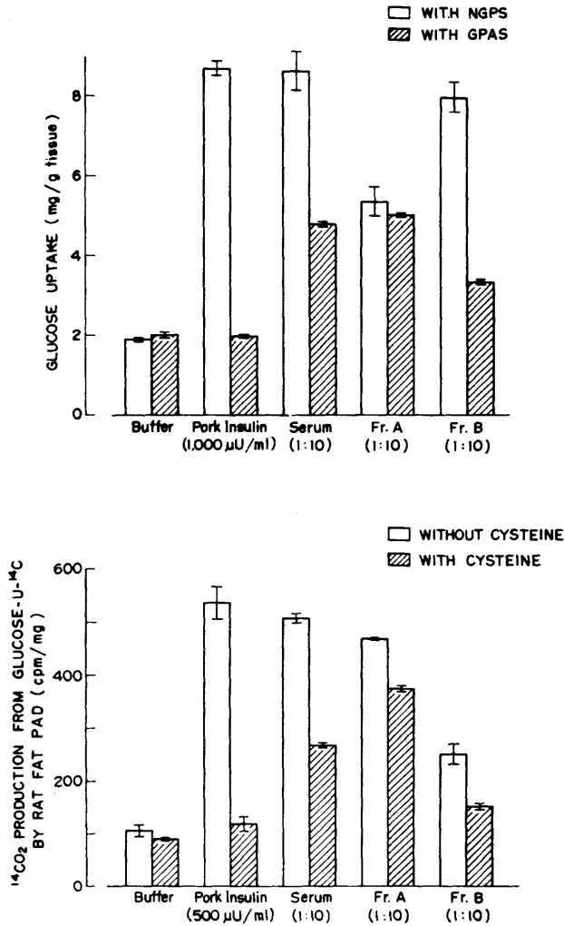
FIG. 4. Suppression of effects of insulin, serum, Fractions A and B by anti-insulin serum or by cysteine treatment. Each bar represents the mean of duplicate estimations. Above: Normal guinea pig serum (NGPS) was added to control flasks. Addition of guinea pig anti-insulin serum (GPAS) completely suppressed the effect of insulin and mostly that of Fr. B, while the effect of Fr. A was not affected by anti-serum and that of serum was partially inhibited. Below: Effects of insulin and of Fr. B were suppressed by cysteine near the basal level, while those of serum and Fr. A were partially suppressed.
