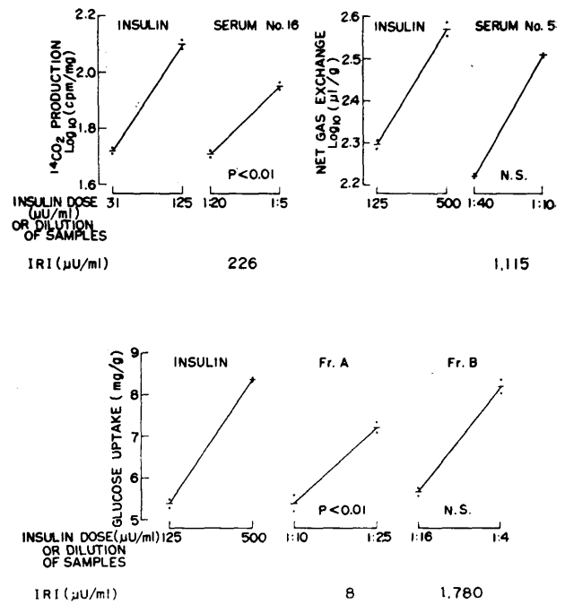
FIG. 5. Test of parallelism between standard insulin and serum or fractions with fat pad assay. Response of fat pad is expressed by C-14-O 2 production from D-glucose-U-C-14 in log 10 (cpm/mg.), net gas exchange in log 10 (μl./gm.), and glucose uptake in mg./gm., respectively, as shown in the figure. When these parameters were measured simultaneously in the same experiments, the ultimate conclusions for parallelism were the same irrespective of different parameters.
