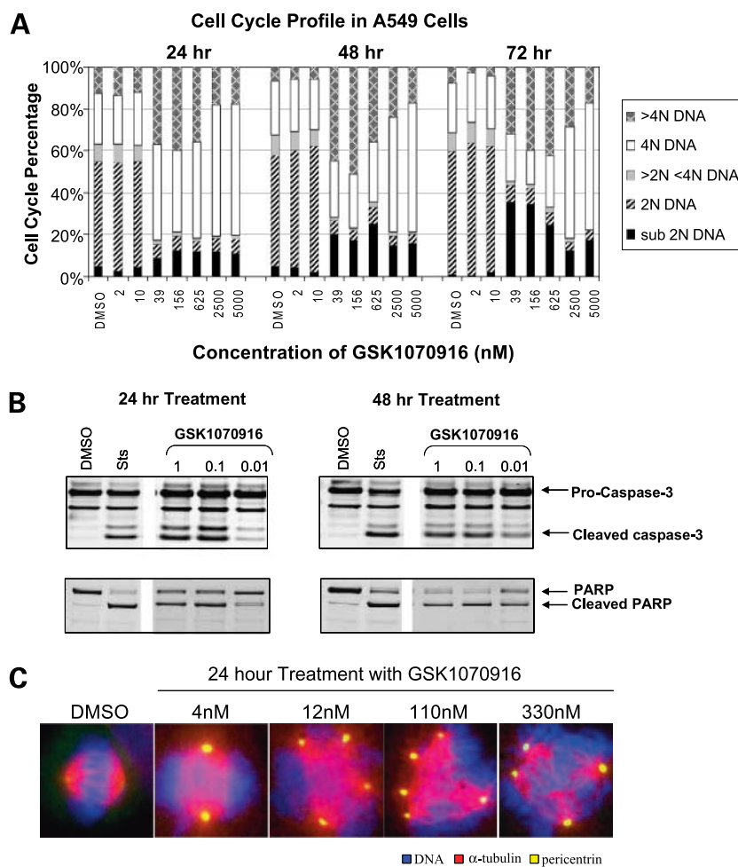
Figure 1. Cellular phenotype after treatment with GSK1070916. A , cell cycle distribution after treatment with GSK1070916. The cell cycle profile was evaluated after 24, 48, or 72 h GSK1070916 treatment by fluorescence-activated cell sorting analysis in A549 cells. A dose-dependent decrease in the 2N DNA content and increases in 4N, >4N, and sub-2N (cell death) DNA compared with DMSO-treated cells were observed. B , induction of Caspase-3 and PARP cleavage by GSK1070916. Colo205 cells were treated with 0.01, 0.1, and 1 \mu mol/L of GSK1070916, 0.1 \mu mol/L of staurosporine ( Sts ) or DMSO for 24 or 48 h. Lysates were analyzed by Western blot analysis using antibodies specific for Caspase-3 and PARP. GSK1070916 induced apoptosis as measured by Caspase-3 and PARP cleavage. C , mitotic phenotype of GSK1070916-treated A549 tumor cells by immunofluorescent staining. A549 cells were treated with 4, 12, 110, or 330 nmol/L of GSK1070916 or DMSO for 24 h and stained with \alpha -tubulin antibody ( red staining ) to visualize mitotic spindles, pericentrin antibodies for centrosomes ( yellow staining ), and 4',6-diamidino-2-phenylindole stained for DNA ( blue staining ). Normal metaphase mitotic structures were observed in the DMSO-treated control cells. Treatment with increasing concentrations of GSK1070916 resulted in unorganized chromosomes as well as the formation of malformed bipolar and multipolar spindles with multipolar spindles being the predominant phenotype.
