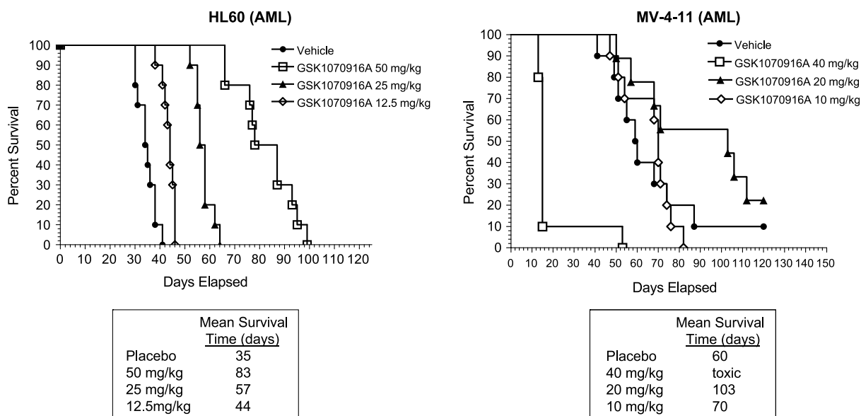
Figure 4. Antitumor activity of GSK1070916 in human leukemia mouse models. For AML, SCID (HL60), and NOD-SCID (MV-4-11) mouse leukemia models, the mice ( n = 10 per group) were treated i.p. with GSK1070916 at 12.5, 25, or 50 mg/kg or 10, 20, or 40 mg/kg, respectively. GSK1070916 was given once daily for 5 consecutive d with 2 d off, for two (HL60) or three (MV-4-11) cycles of treatment. A dose-dependent increase in the median survival times was observed after i.p. dosing in the GSK1070916 treated animals compared with the vehicle-treated mice.
