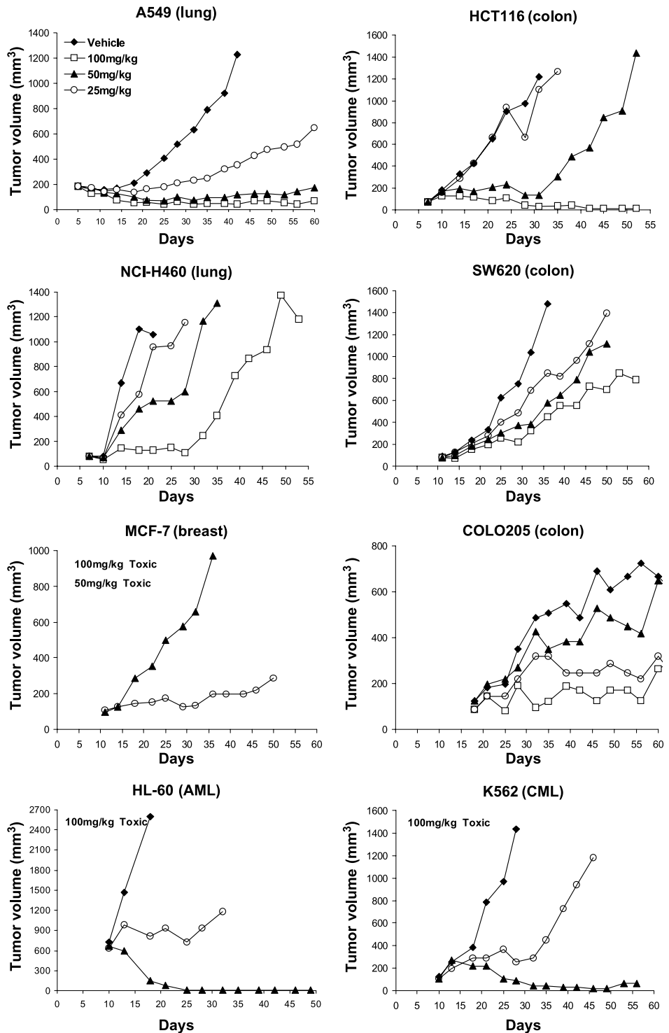
Figure 3. Antitumor activity of GSK1070916A in vivo . GSK1070916A was administered at 25, 50, or 100 mg/kg once daily for 5 consecutive d-on, 2 d-off schedule for two (Colo205 and HL60) or three (A549, SW620, HCT116, H460, MCF-7, K562) cycles. Toxicity is shown for each tumor line where observed.
