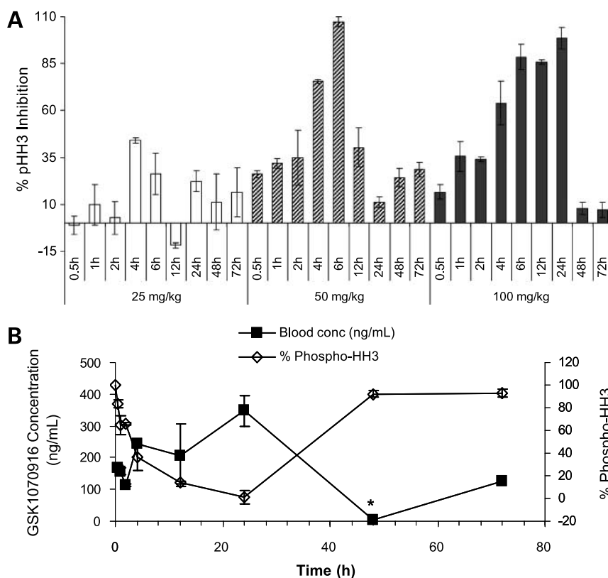
Figure 2. Pharmacodynamic effects and concentrations of GSK1070916. GSK1070916A was administered i.p. as a single dose to nude mice with subcutaneous HCT116 tumors at 25, 50, or 100 mg/kg. A , at the indicated times, pHH3-Ser10 levels in tumors were determined. GSK1070916 inhibited HH3-S10 phosphorylation in a dose-dependent manner at all three doses. B , after a single i.p. dose of 100 mg/kg of GSK1070916, drug concentrations were measured in blood and HCT116 tumor tissues. Blood concentrations of >170 ng/mL of GSK1070916 correlated with sustained decrease (>60%) in HH3-S10 phosphorylation for up to 24 h. *, the concentration of GSK1070916 in the blood at 48 h was below the lower limit of quantification in this assay. A value of 5 ng/mL that is one half the lower limit of quantification was therefore used to not over represent the concentration in the graph. The levels of GSK1070916 in tumor samples after a single administration were below the level of detection in this study.
